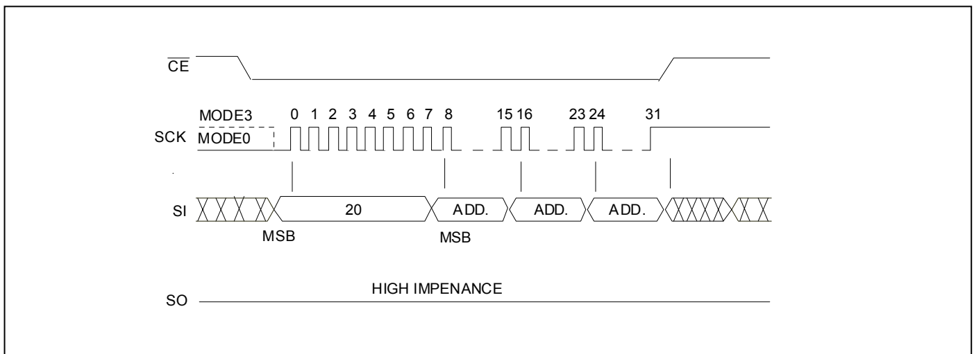
FIGURE 10 : SEQUENCE-ERASE SEQUENCE
