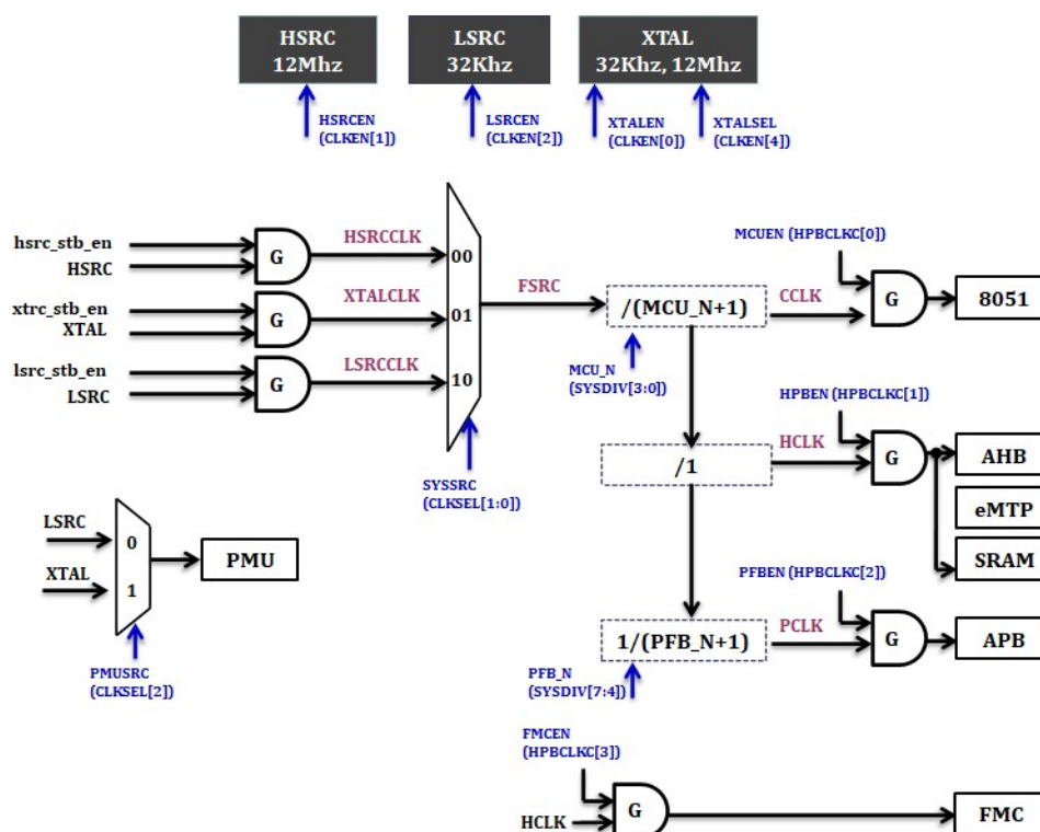
Figure 6.5-1 Clock Architecture of HPB Peripherals
