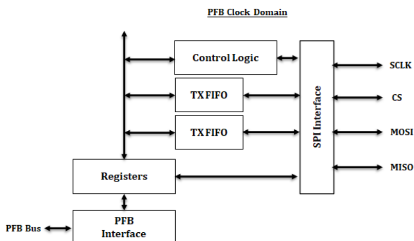
Figure 6.15-1 SPI Controller Block Diagram
