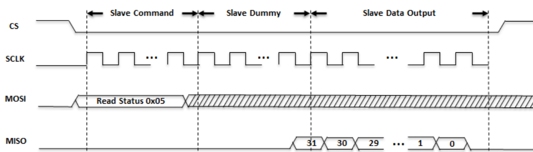
Figure 6.15-3 Timing Diagram of Read Slave Status Command
