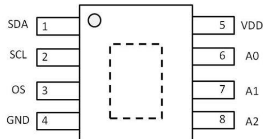
Topside view of ETS75A
