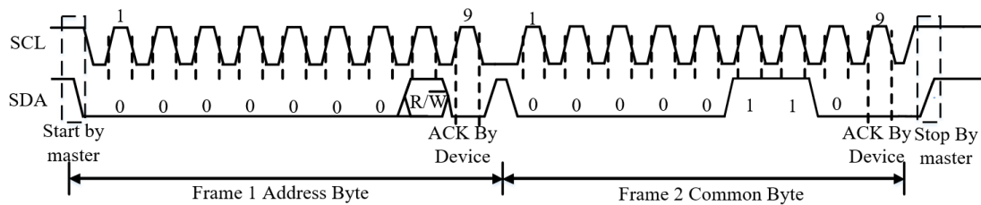
Figure. General-Call Reset Command Timing Diagram
