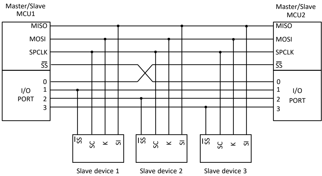
Fig 22.5-1 Multi-master/multi-slave mode
