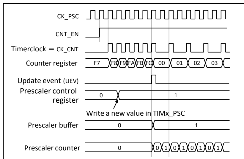
Fig 10.1-2 Counter timing diagram with prescaler division change from 1 to 2
