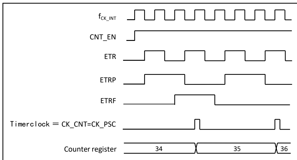
Fig 10.1-26 Control circuit in external clock mode 2
