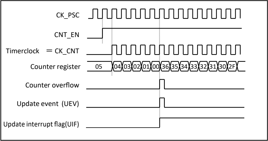
Fig 10.1-10 Counter timing diagram, internal clock divided by 1
