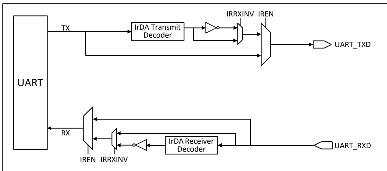
Fig 19.4-1 IrDA Diagram
