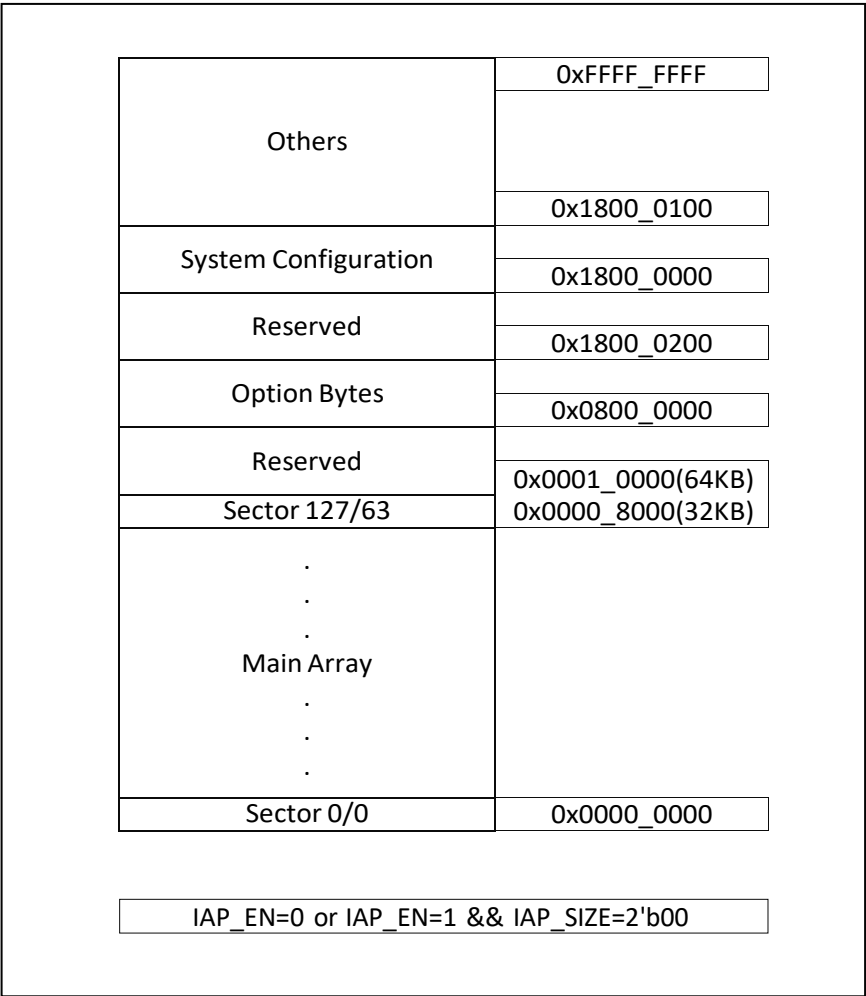
Fig 3.3-1 Boot area address mapping
