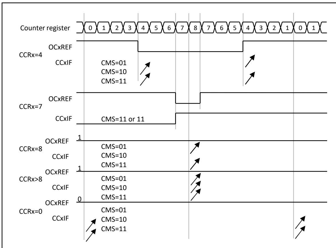
Fig 10.1-34 Center-aligned PWM waveforms (ARR=8)
