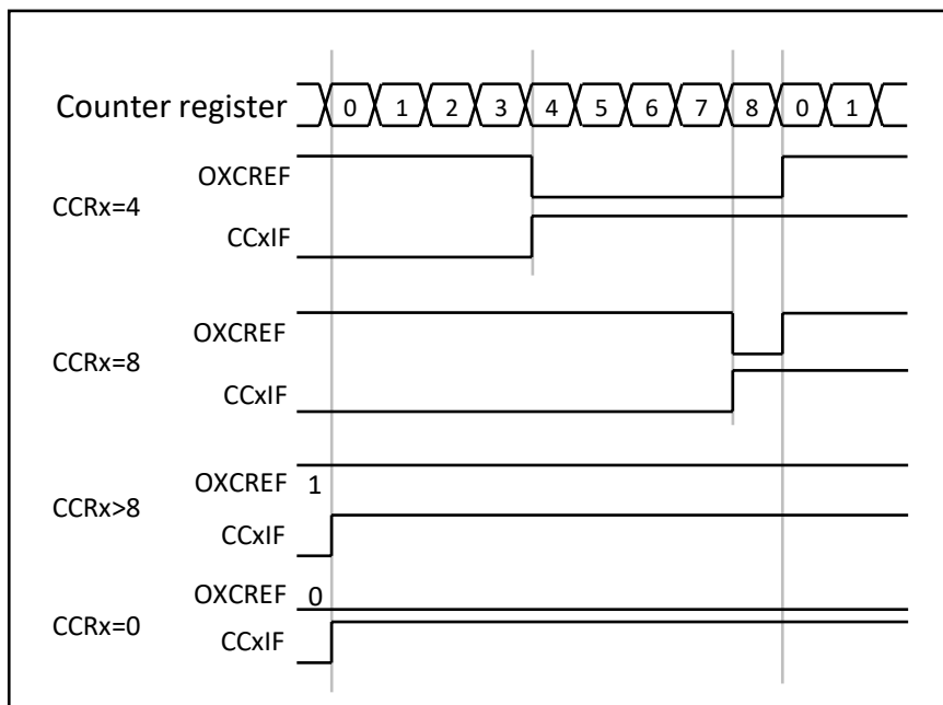
Fig 10.1-33 Edge-aligned PWM waveforms (ARR=8)
