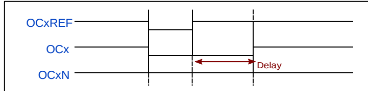
Fig 10.1-36 Dead-time waveforms with delay greater than the negative pulse.
