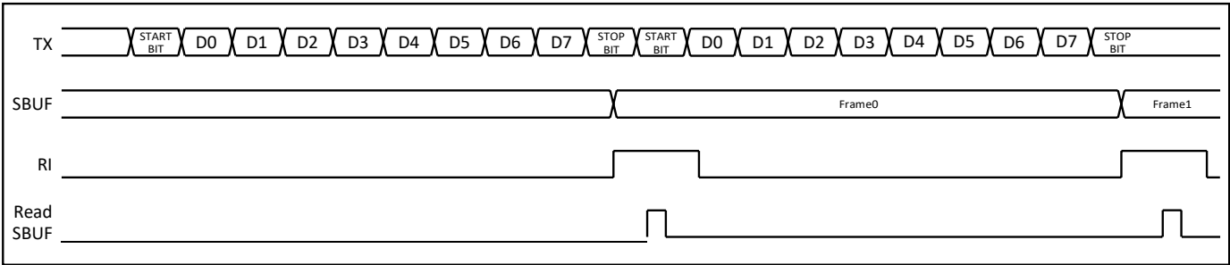
Fig 20.10-1 Receive buffer
