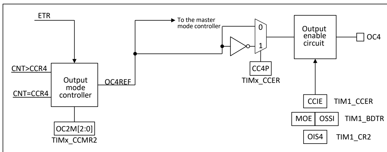
Fig 10.1-30 Output stage of capture/compare channel (channel 4)
