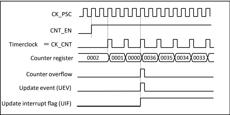
Fig 10.1-11 Counter timing diagram, internal clock divided by 2
