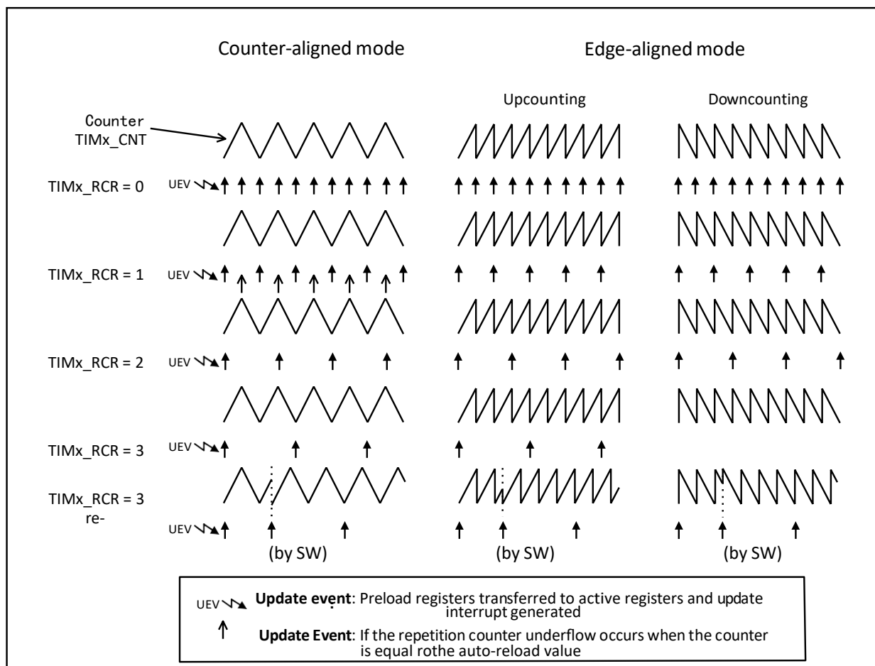
Fig 10.1-21 Update rate examples depending on mode and TIM1_RCR register settings
