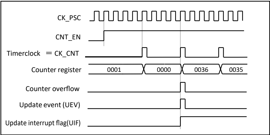
Fig 10.1-12 Counter timing diagram, internal clock divided by 4
