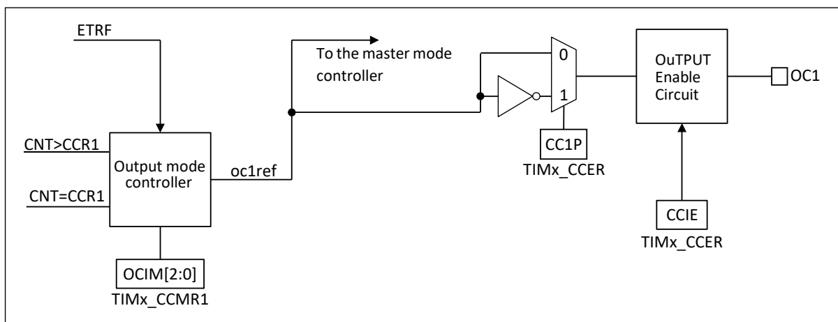
Fig 11.3-27 Capture/compare channel (example: channel 1 output stage)
