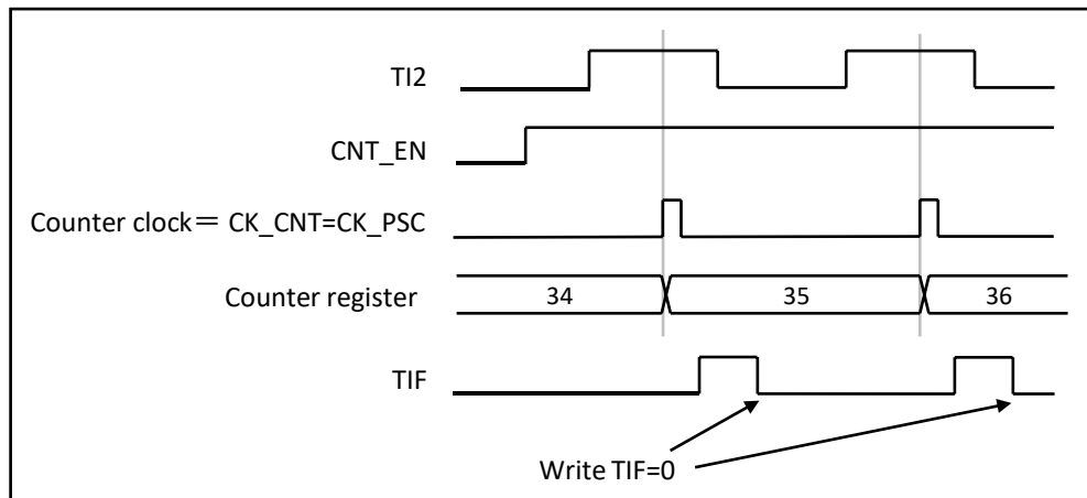
Fig 11.3-22 T12 control circuit in external clock mode 1
