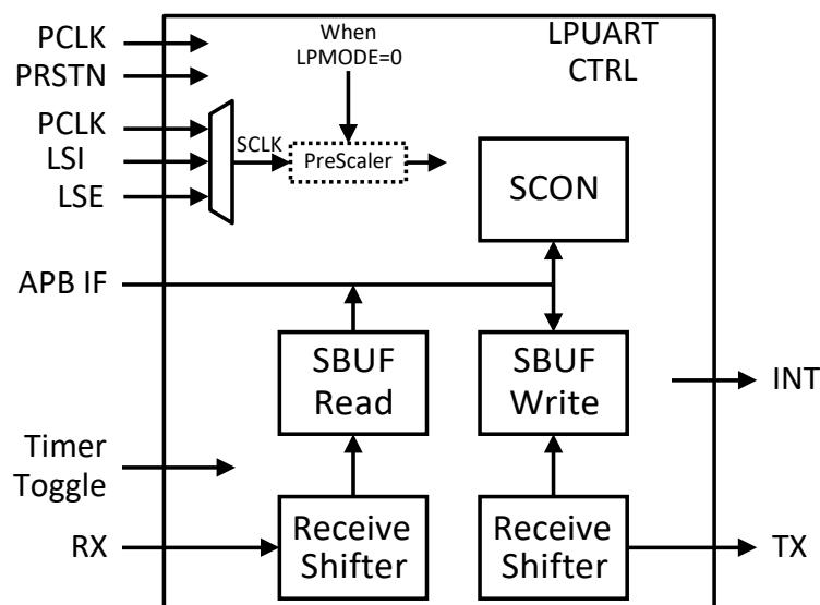
Fig 20.2-1 LPUART Block Diagram
