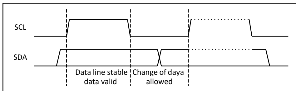
Fig 21.3-5 I2C bus transmission
