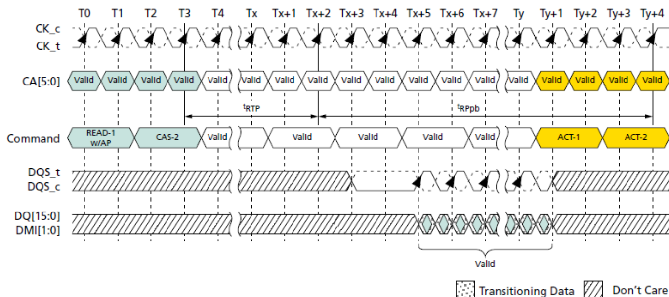
Burst READ With Auto Precharge – BL16, Non-Toggling Preamble, 0.5nCK Postamble
