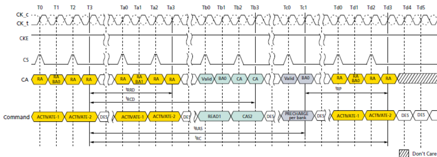
ACTIVATE Command
