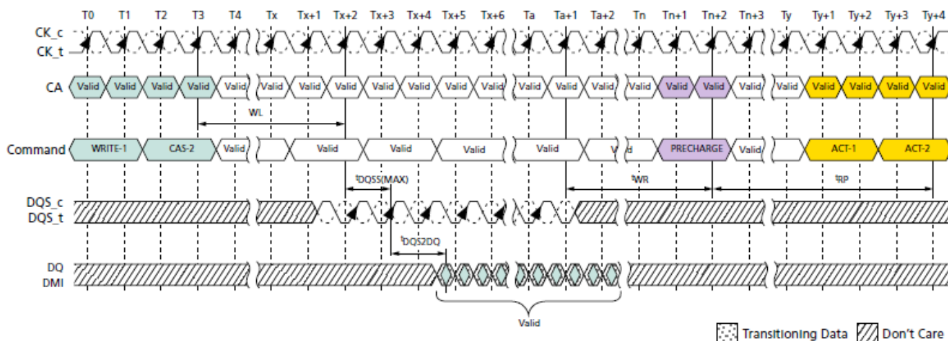
Burst WRITE Followed by PRECHARGE – BL16, 2nCK Preamble, 0.5nCK Postamble
