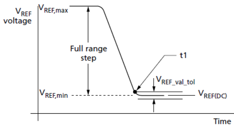
V REF(DQ) Full Step from V REF,max to V REF,min
