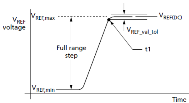
V REF(DQ) Full Step from V REF,min to V REF,max
