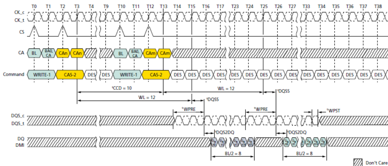
Consecutive WRITE: t_{CCD} = \text{MIN} + 2, 0.5n\text{CK} Postamble
