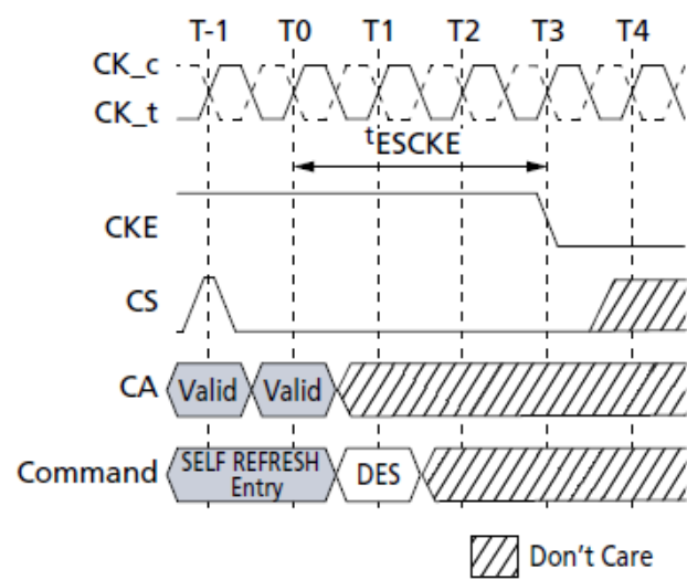
tESCKE Timing
