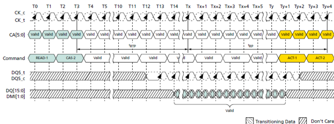
Burst READ With Auto Precharge – BL32, Toggling Preamble, 1.5nCK Postamble
