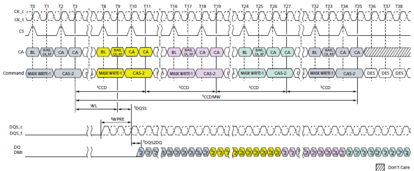
MASK WRITE Command – Different Bank
