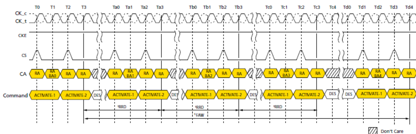
t_{FAW} Timing
