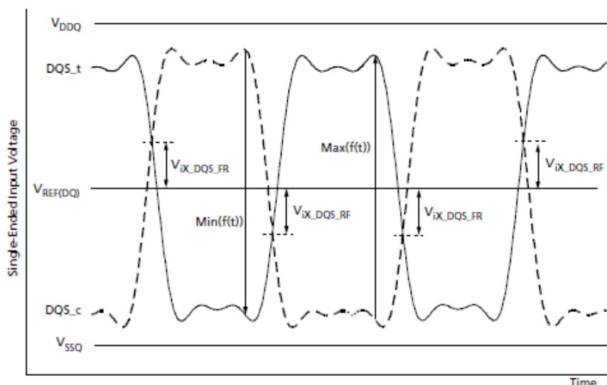
V_{ix} Definition (DQS)
