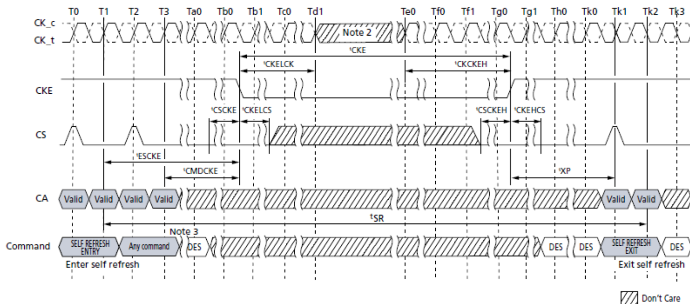
Self Refresh Entry/Exit Timing with Power-Down Entry/Exit
