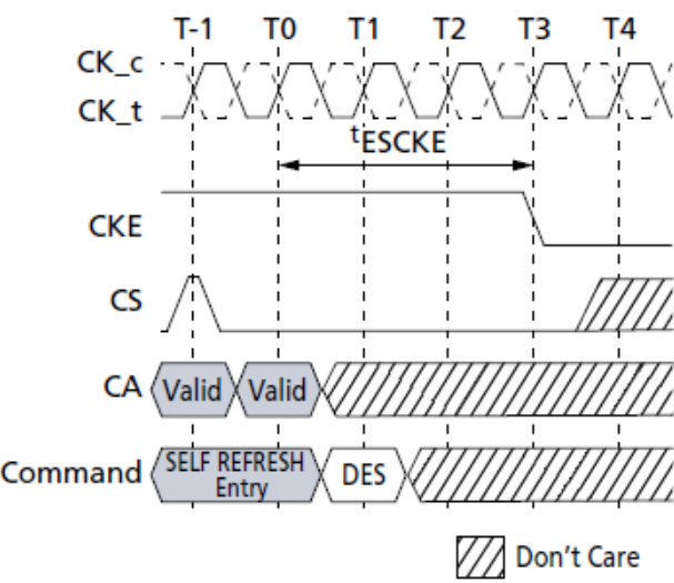
t_{ESCKE} Timing
