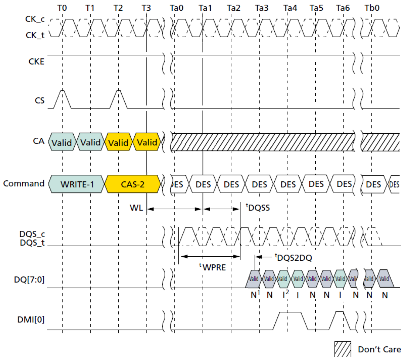
WRITE Command with Write DBI Enabled; DM Disabled
