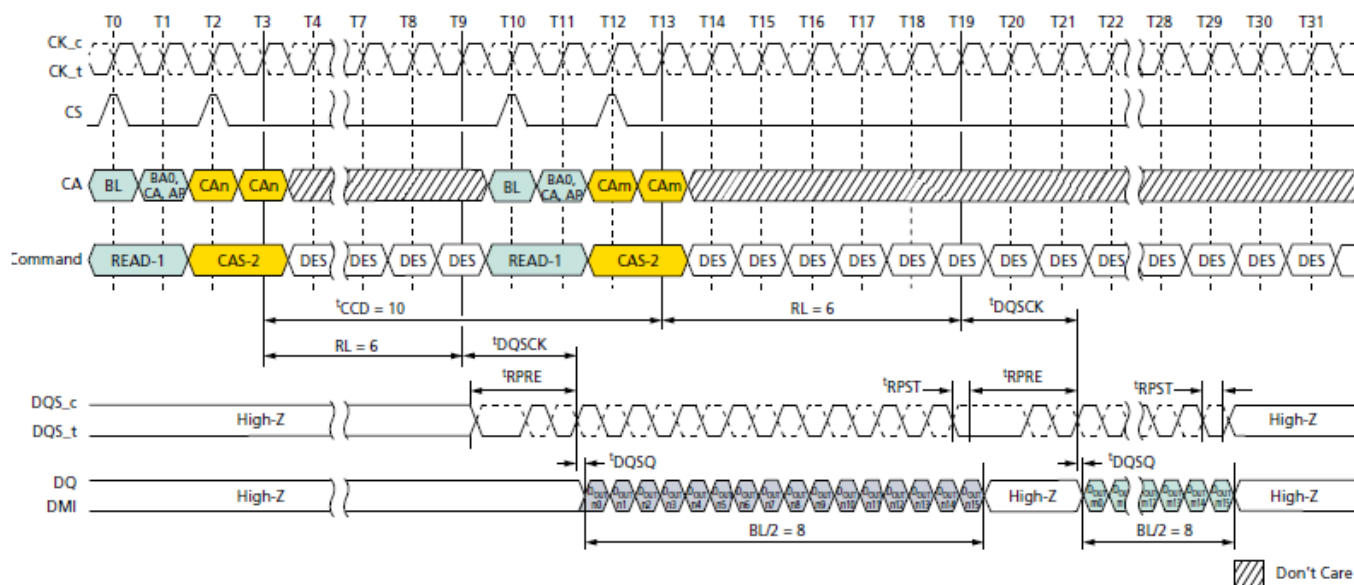
Consecutive READ: t_{CCD} = \text{MIN} + 2 , Preamble = Toggle, 0.5nCK Postamble
