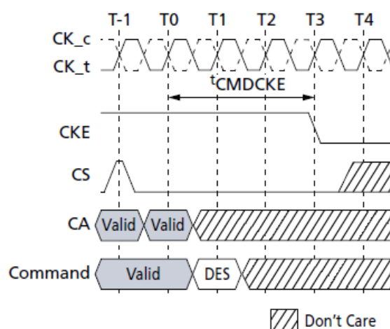
t_{CMDCKE} Timing
