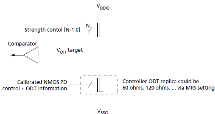
Pull-Up Calibration
