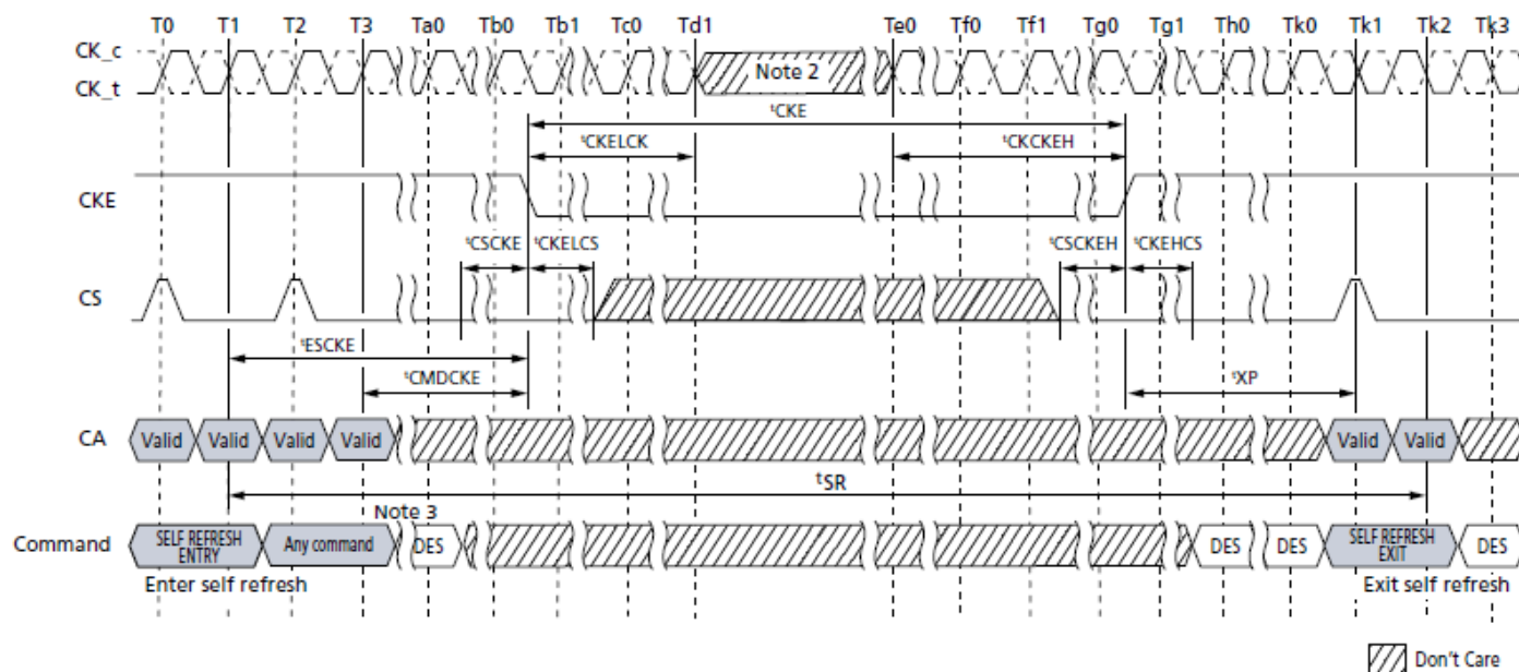
Self Refresh Entry/Exit Timing with Power-Down Entry/Exit
