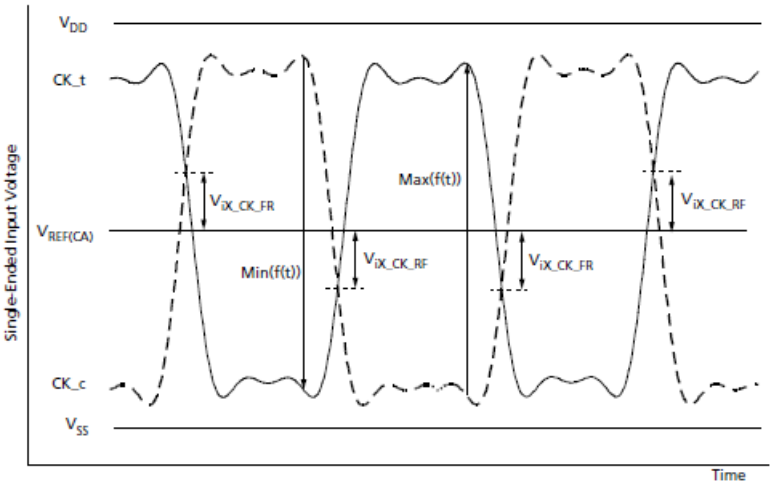
V_{ix} Definition (Clock)
