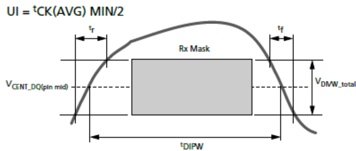
DQ t_{DIPW} and SRIN_divW Definition for Each Input Pulse
