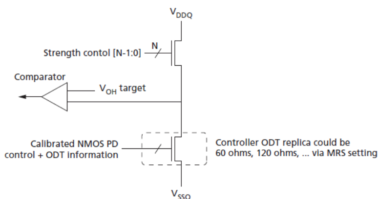
Pull-Up Calibration
