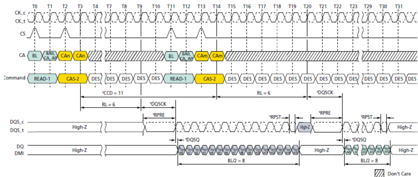
Consecutive READ: t'_{CCD} = \text{MIN} + 3 , Preamble = Static, 0.5n\text{CK} Postamble
