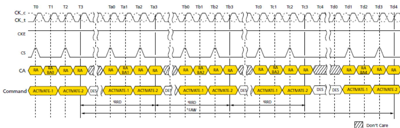
t FAW Timing
