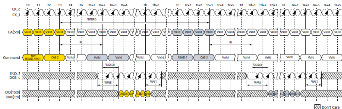
READ-FIFO – t_{RPRE} = \text{Toggleing} , t_{RPST} = 1.5nCK
