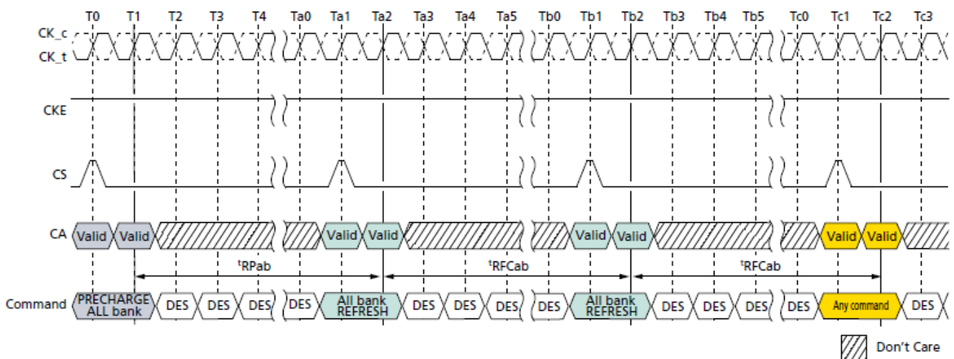
All-Bank REFRESH Operation
