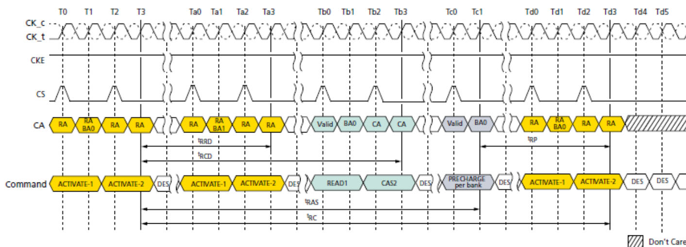
ACTIVATE Command
