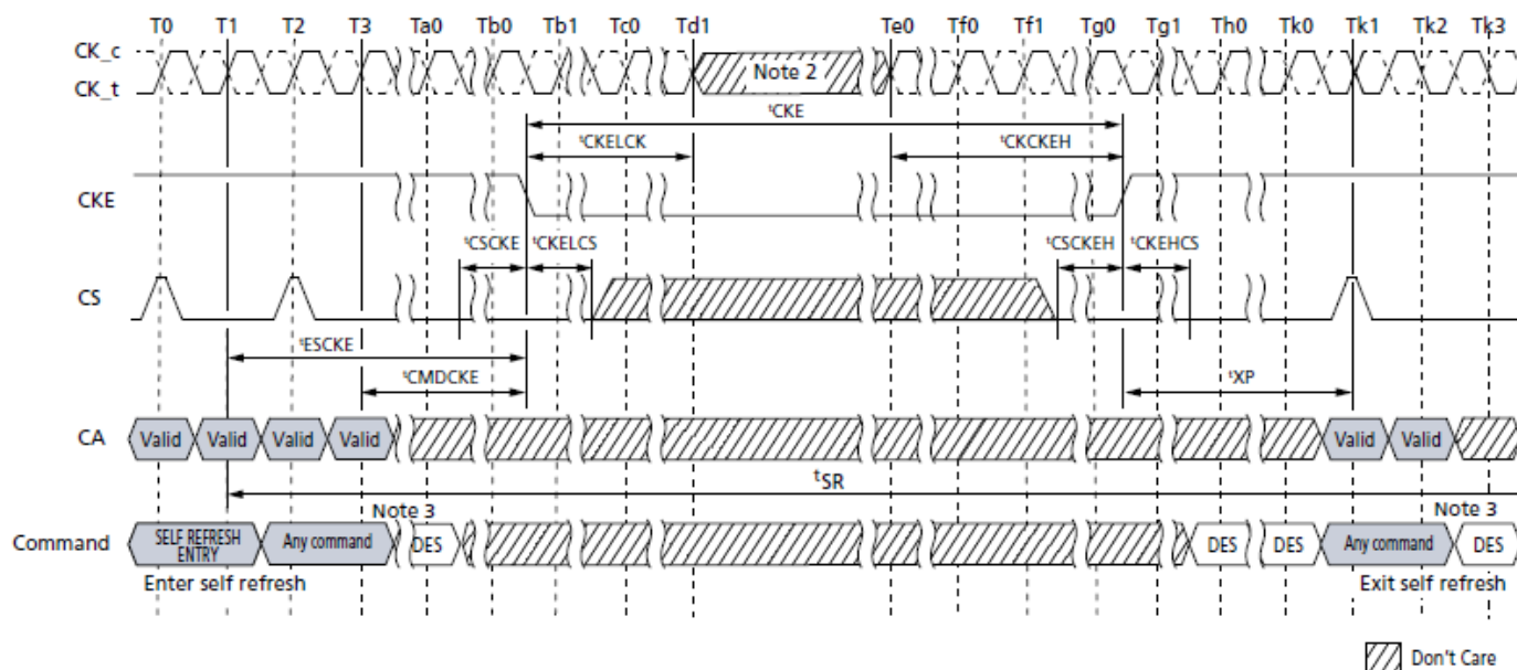
Command Input Timings after Power-Down Exit During Self Refresh
