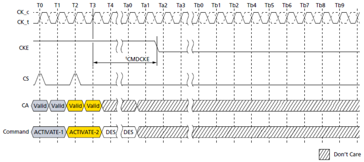
ACTIVATE Command to Power-Down Entry
