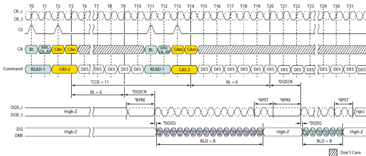
Consecutive READ: t'_{CCD} = \text{MIN} + 3 , Preamble = Static, 1.5n\text{CK} Postamble
