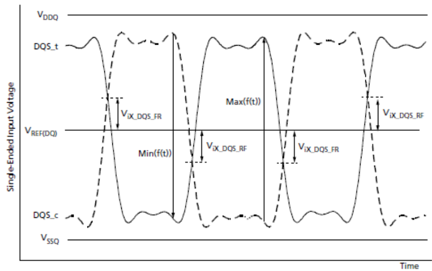
V_{ix} Definition (DQS)
