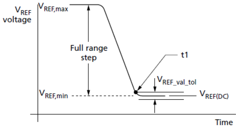
V_{REF(CA)} Full Step from V_{REF,max} to V_{REF,min}
