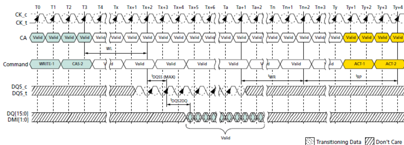
Burst WRITE With Auto Precharge – BL16, 2nCK Preamble, 0.5nCK Postamble
