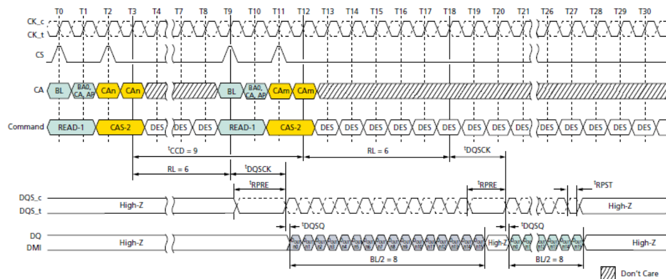
Consecutive READ: t_{CCD} = \text{MIN} + 1 , Preamble = Static, 0.5nCK Postamble
