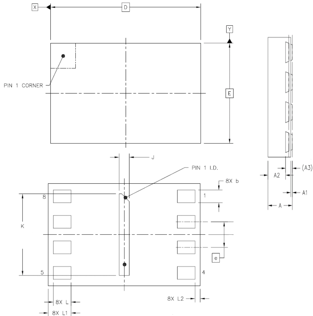
Figure 40. USON8 2x3x0.55mm
