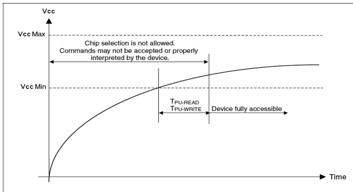
Figure 32. Power-up Timing
