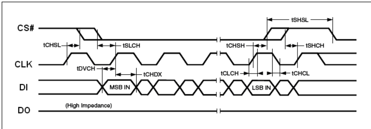
Figure 35. Input Timing
