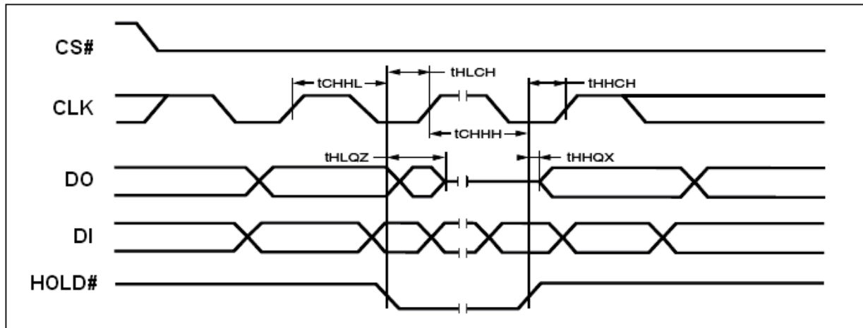
Figure 36. Hold Timing
