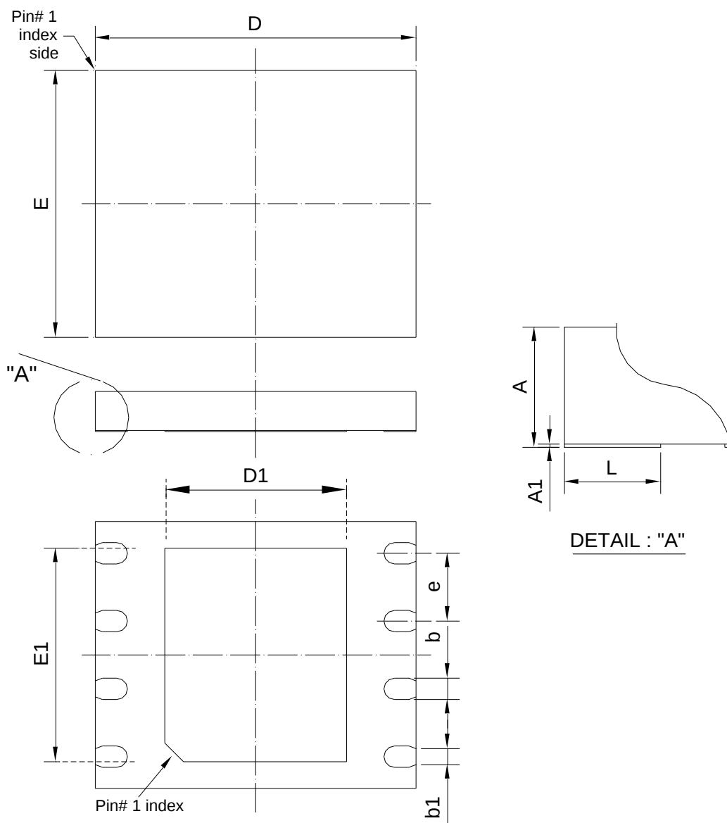
Figure 42. VDFN / WSON 8 5x6mm
