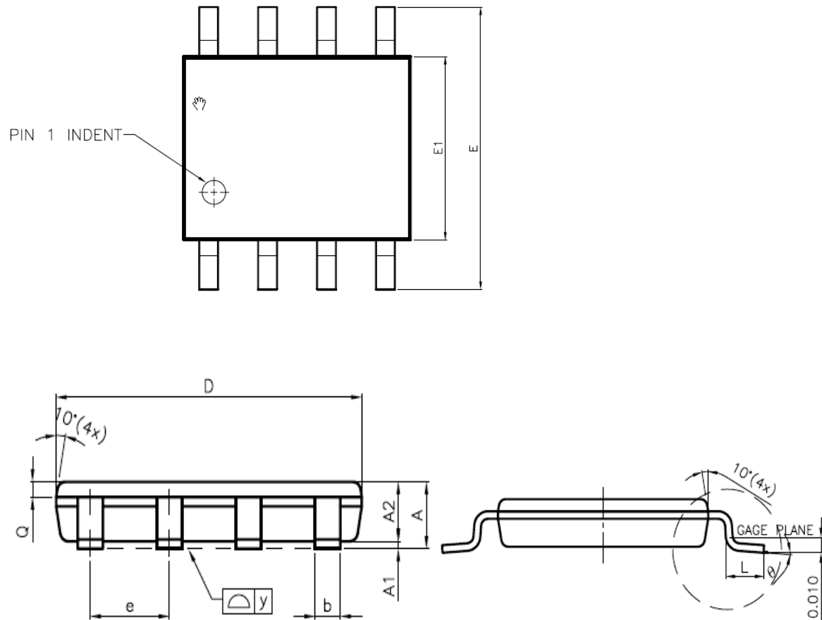
Figure 39. VSOP8 150mil
