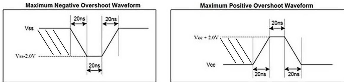
Figure 114. Overshoot Waveform
