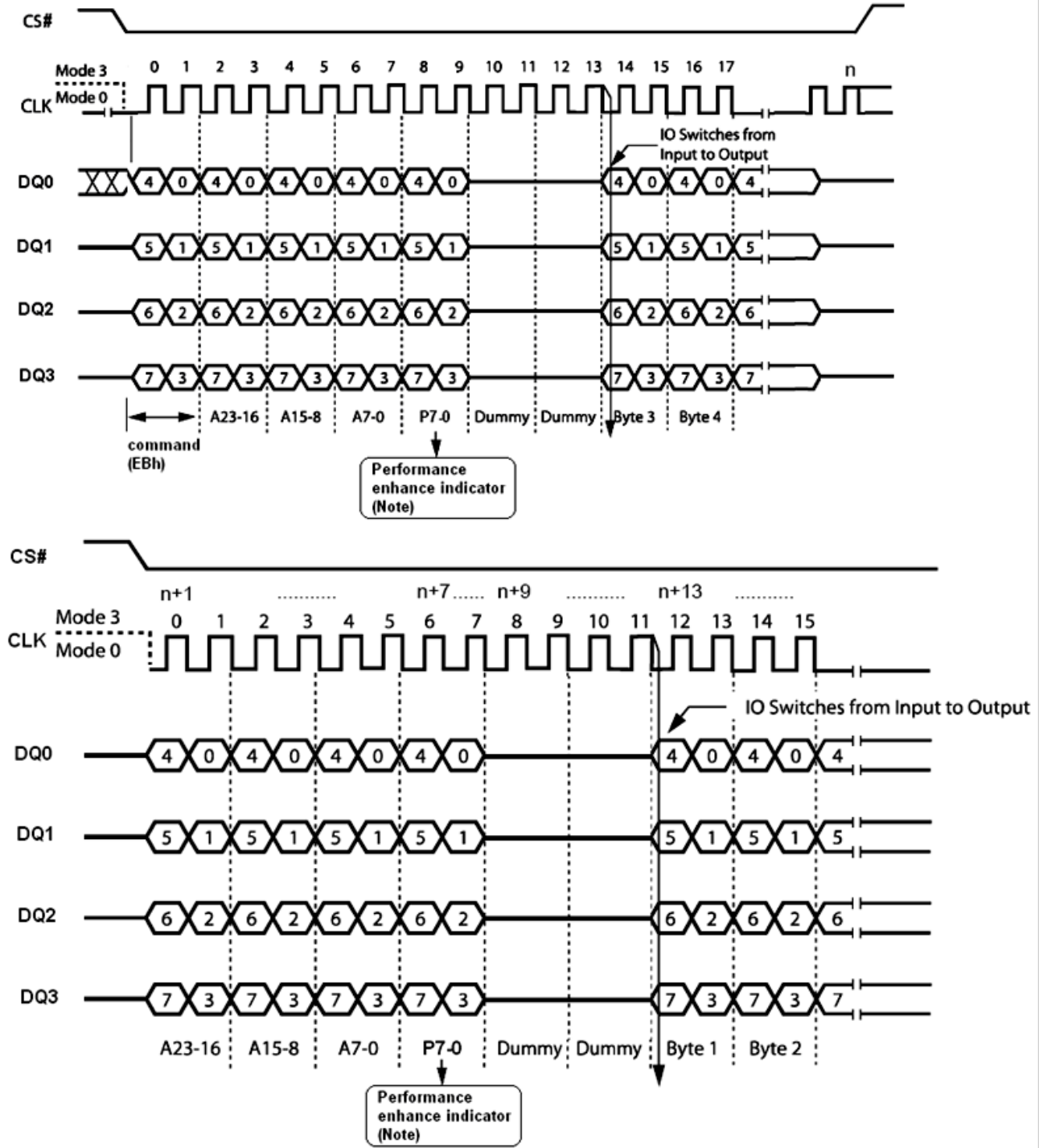
Figure 42. Quad Input/ Output Fast Read Enhance Performance Mode Sequence in QPI Mode
