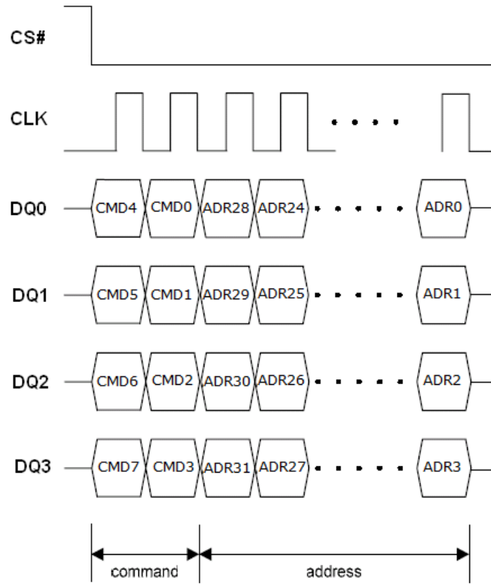
Figure 80. Block/Sector Erase with 4byte address Instruction Sequence in QPI Mode
