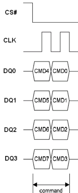
Figure 12. Write Enable/Disable Instruction Sequence under QPI Mode
