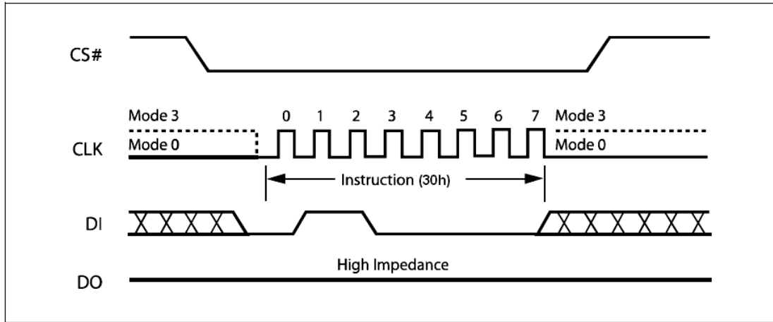
Figure 70. Write Resume Instruction Sequence Diagram
