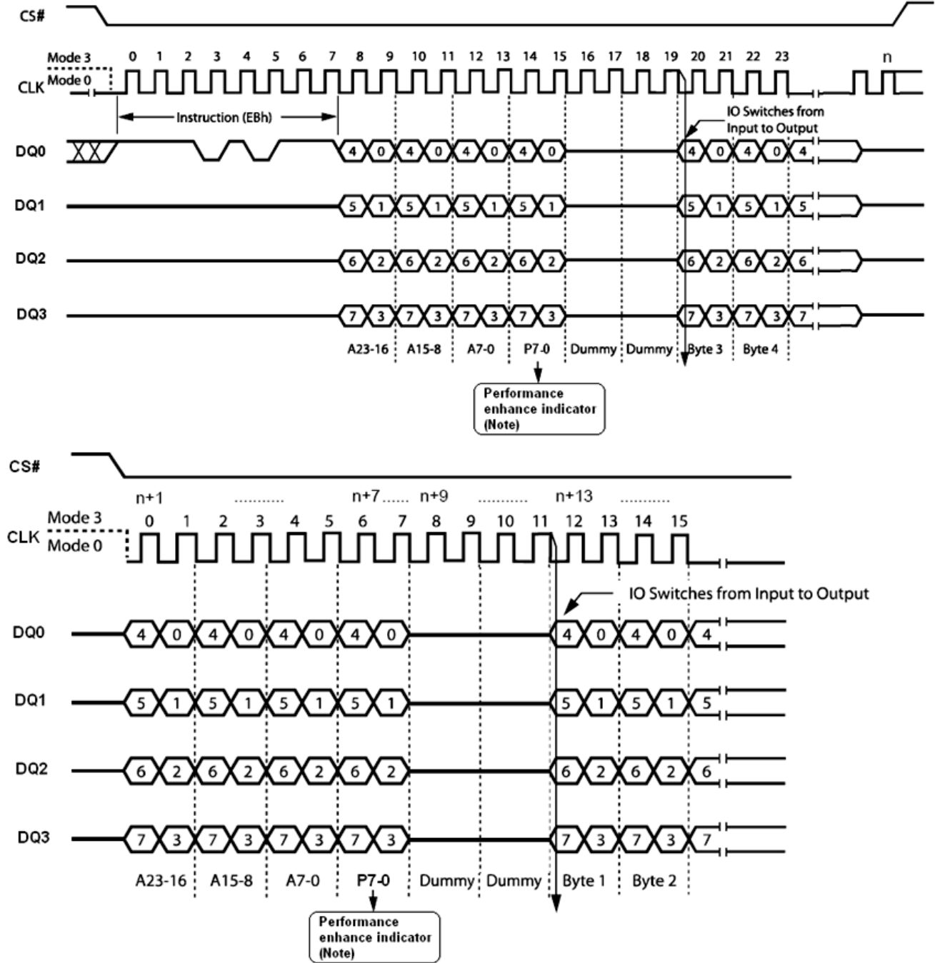
Figure 41. Quad Input/ Output Fast Read Enhance Performance Mode Sequence Diagram
