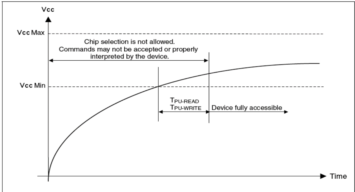
Figure 107. Power-up Timing
