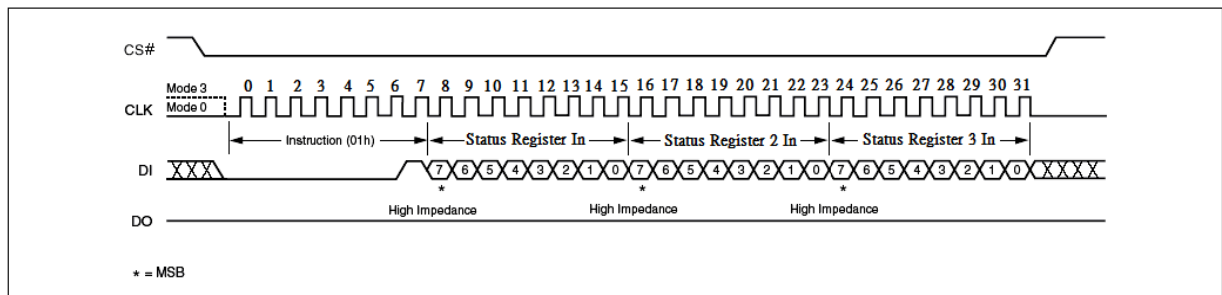
Figure 20. Write Status Register Instruction Sequence Diagram (multi byte)
