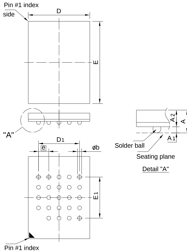
Figure 119. TFBGA24 6x8 mm (5x5-1)
