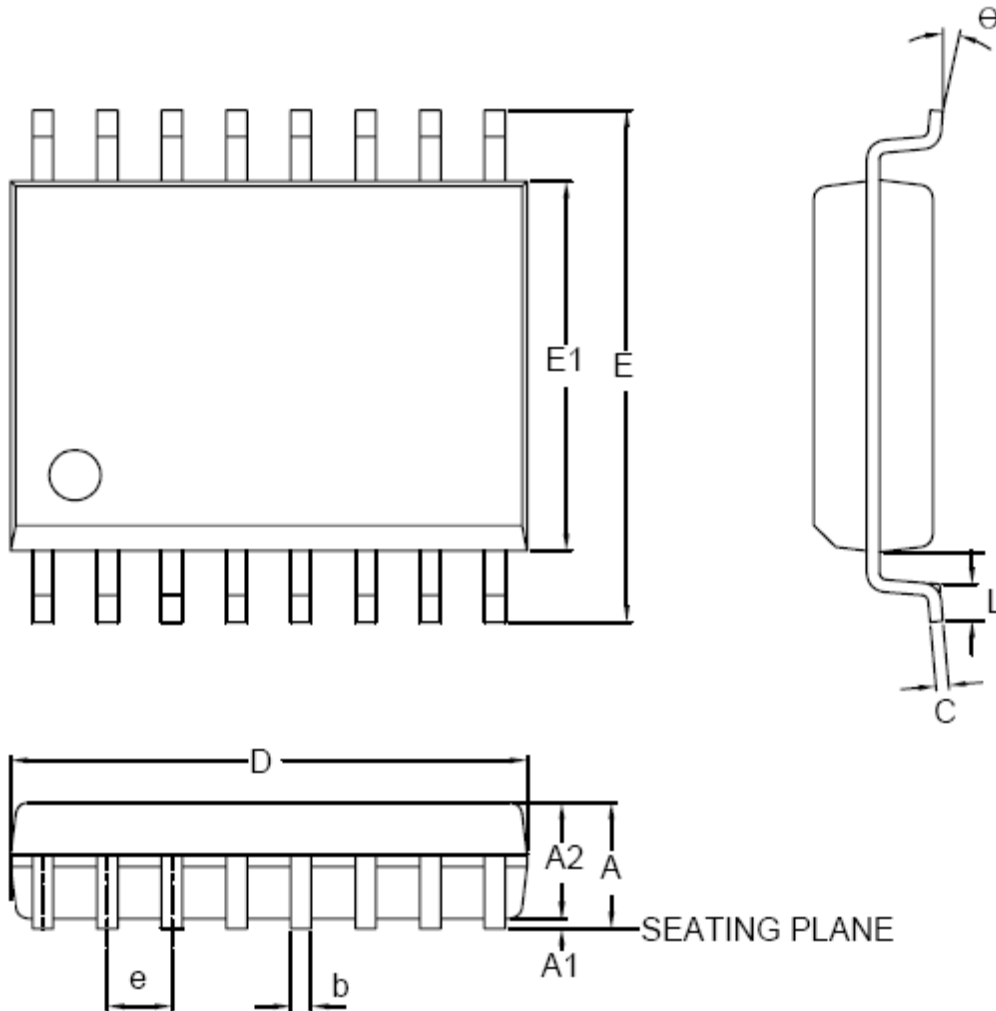
Figure 118. SOP16 300 mil
