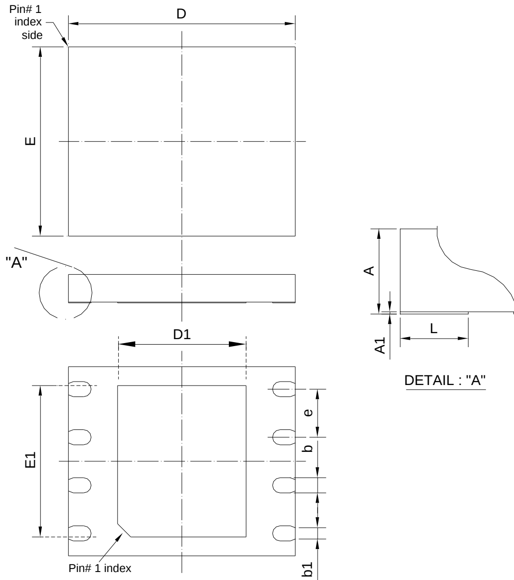
Figure 116. VDFN / WSON8 5x6 mm
