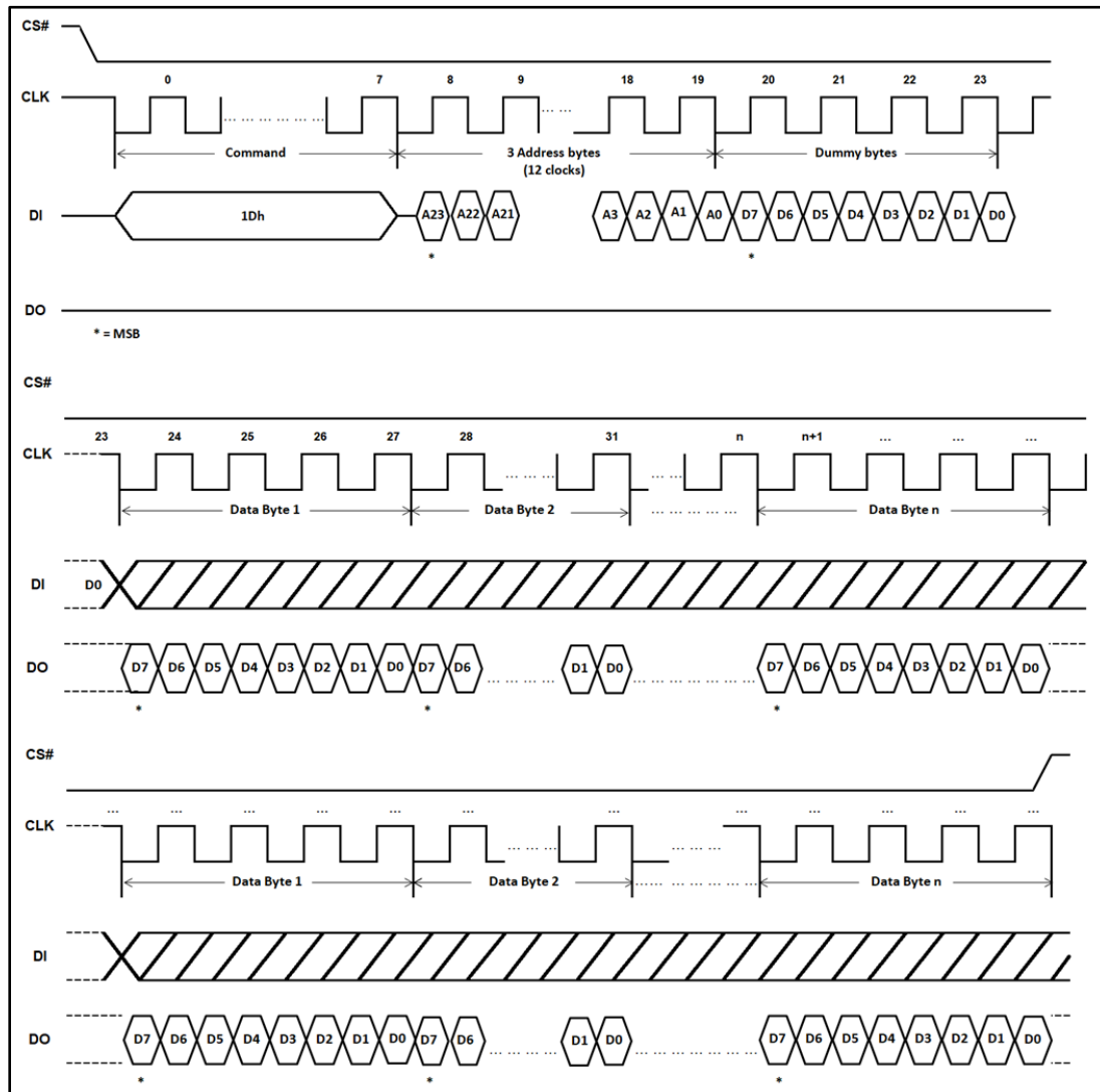
Figure 57. DDR Read Burst with Wrap Instruction Sequence Diagram
