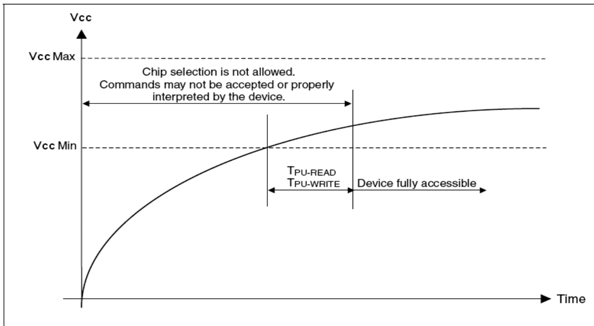
Figure 108. Power-up Timing
