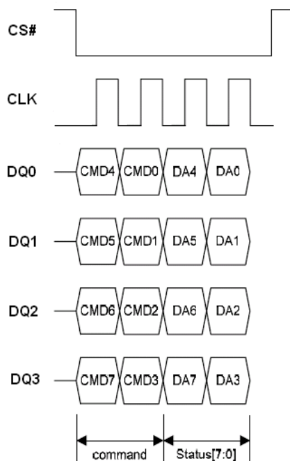
Figure 91. Write Extended Register Instruction Sequence in QPI Mode
