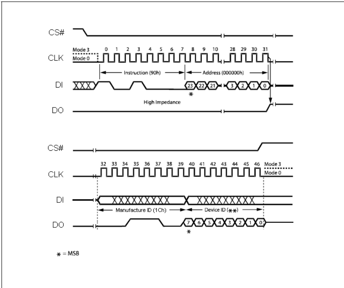
Read Manufacturer / Device ID Diagram
