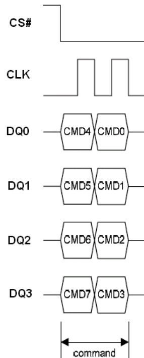
Write Suspend/Resume Instruction Sequence in QPI Mode
