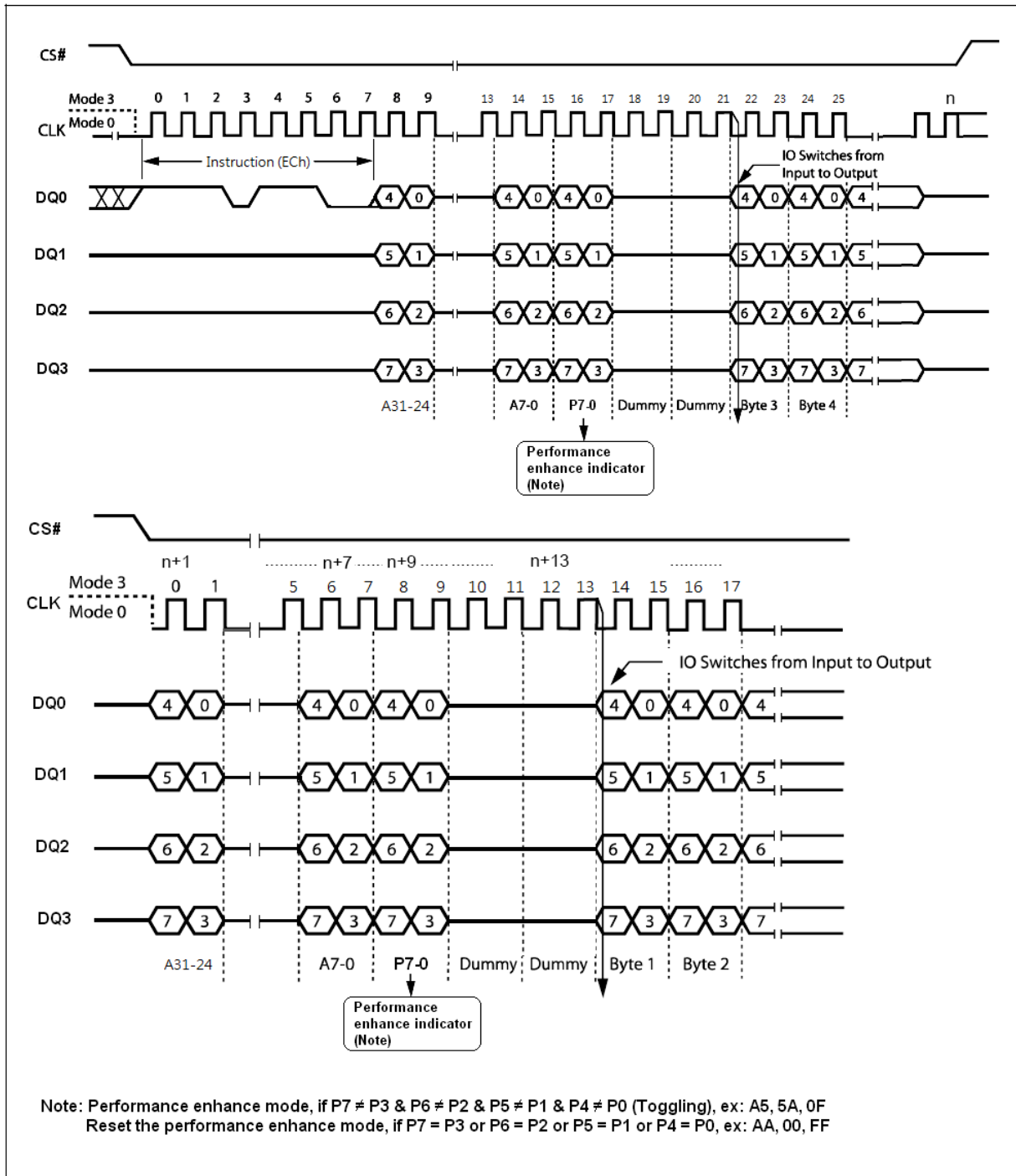
Quad Input/ Output Fast Read Enhance Performance Mode with 4byte address Sequence Diagram
