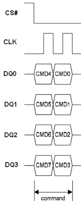
Write Enable/Disable Instruction Sequence under QPI Mode
