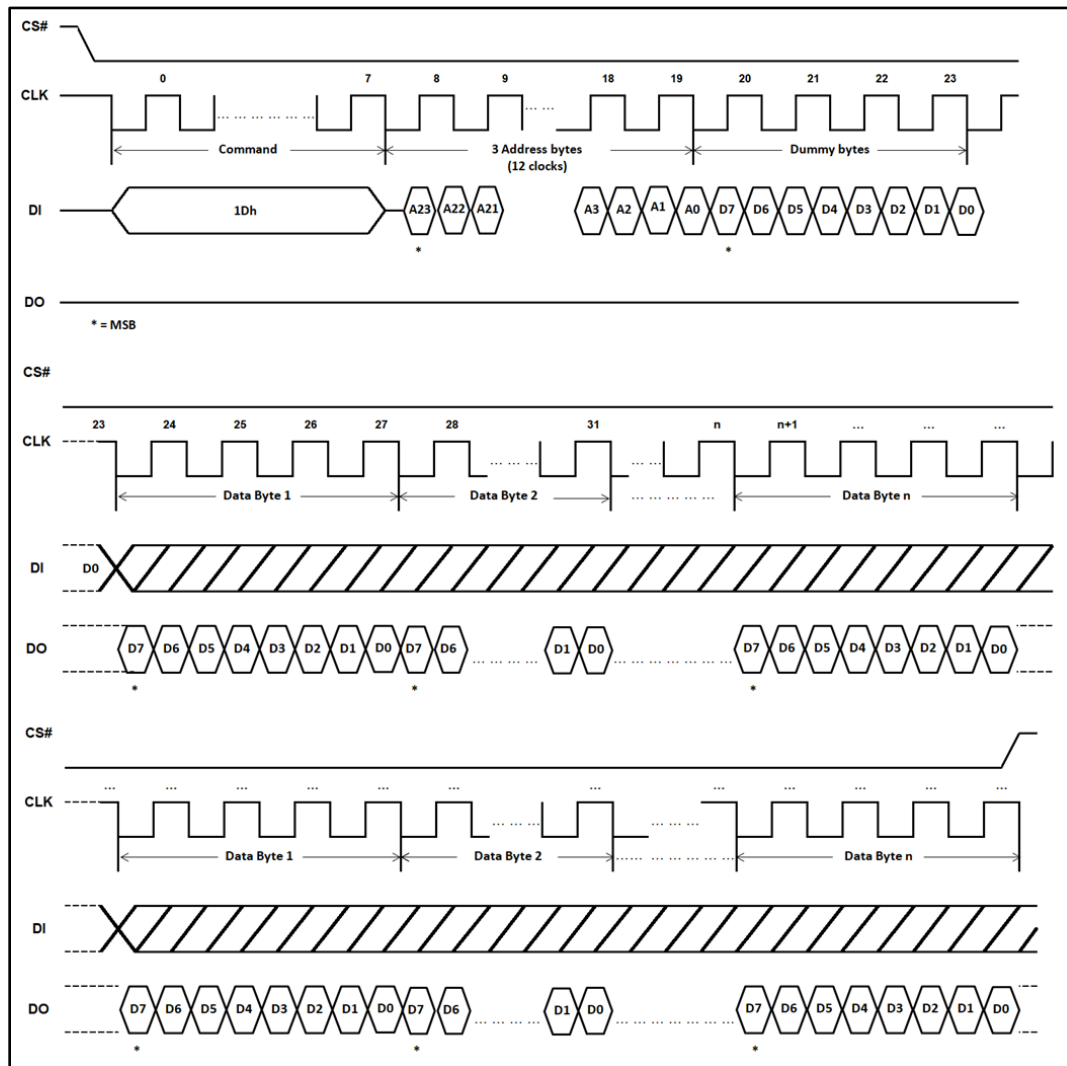
DDR Read Burst with Wrap Instruction Sequence Diagram
