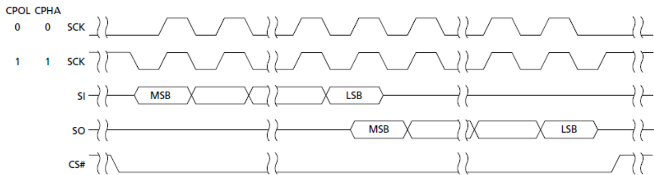
SPI Modes Timing
