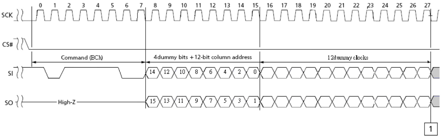
Fast Read x2 IO with 4Byte Address (BCh) Timing
