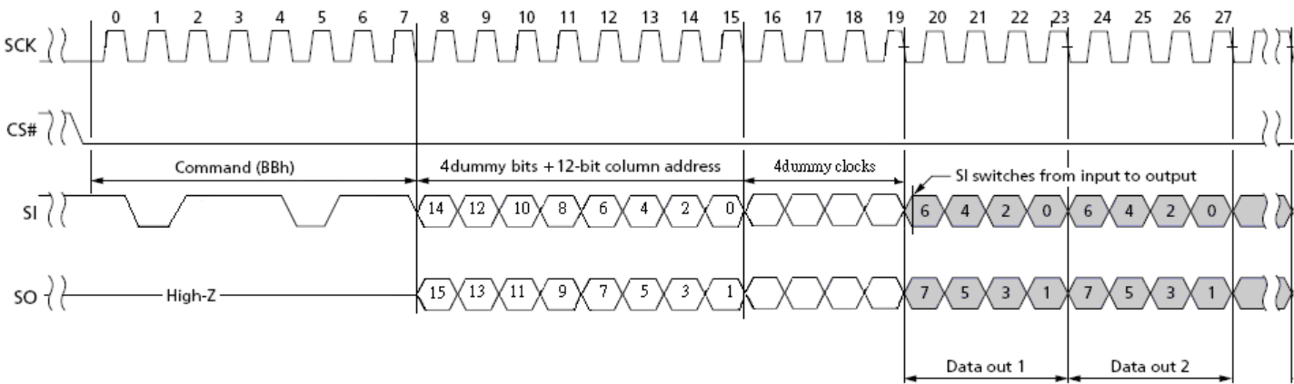
Fast Read x2 IO (BBh) Timing
