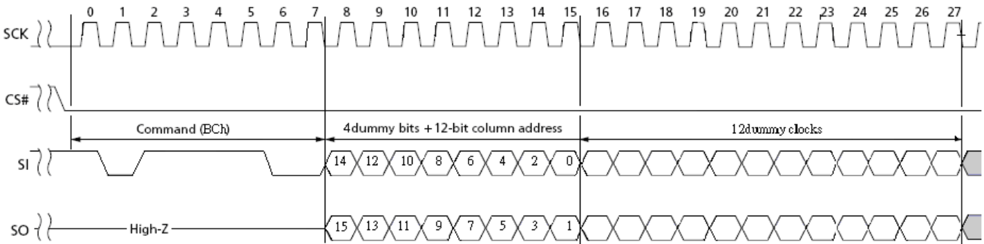
Fast Read X2 IO with 4Byte Address (BCh) Timing
