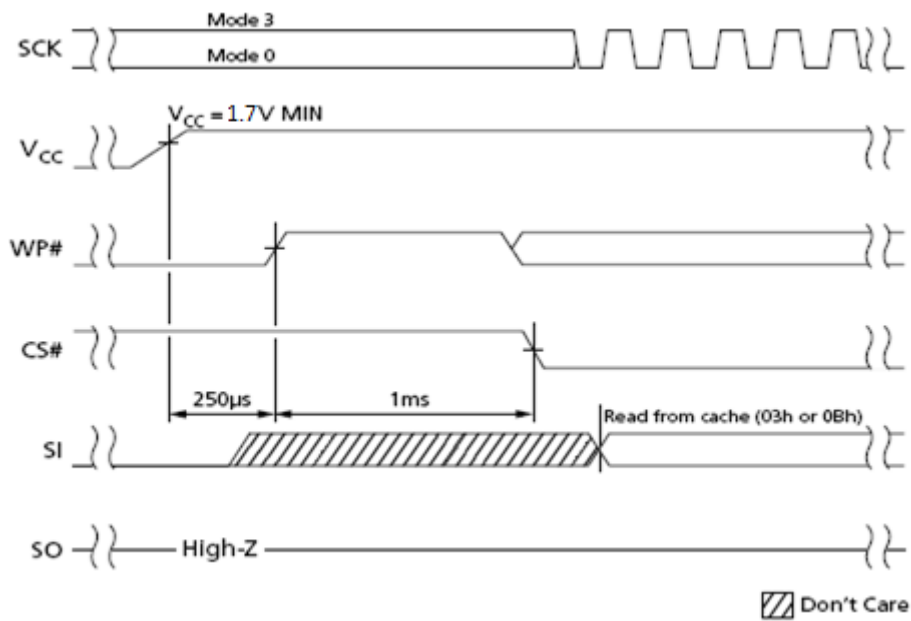
Power-Up and RESET Timing
