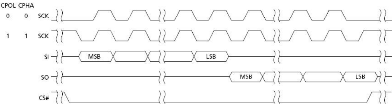
SPI Modes Timing
