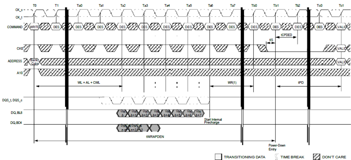
Power-Down Entry After Write with Auto Precharge
