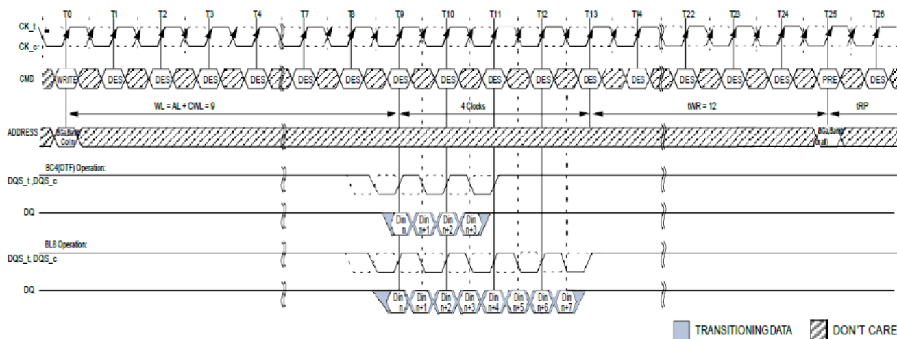
WRITE (BL8/BC4) OTF to PRECHARGE Operation with 1tCK Preamble
