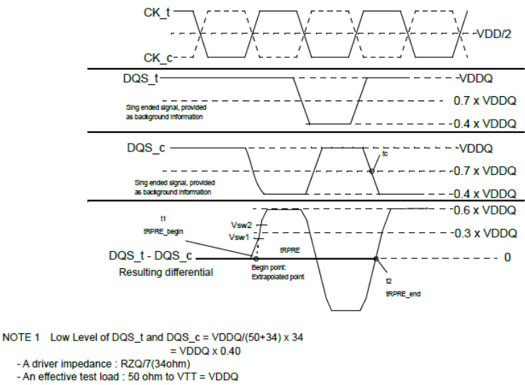
Method for calculating tRPRE transitions and endpoints
