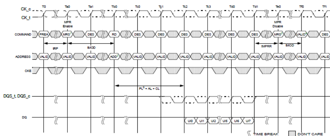
MPR Read Timing
