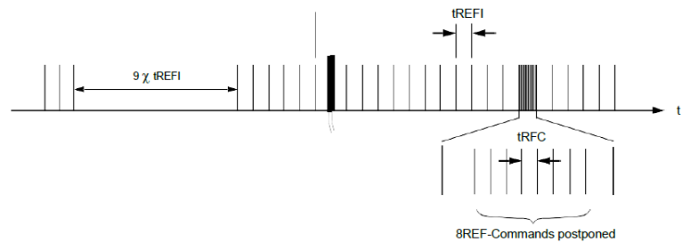
Postponing Refresh Commands (Example of 1X Refresh mode)
