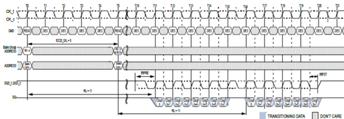
Nonconsecutive READ (BL8) with 1tCK Preamble in Same or Different Bank Group
