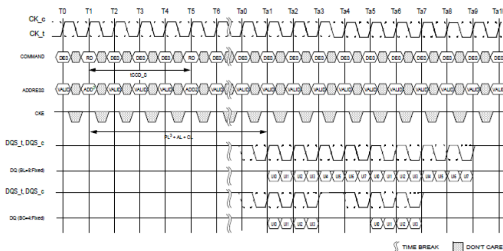
MPR Back to Back Read Timing
