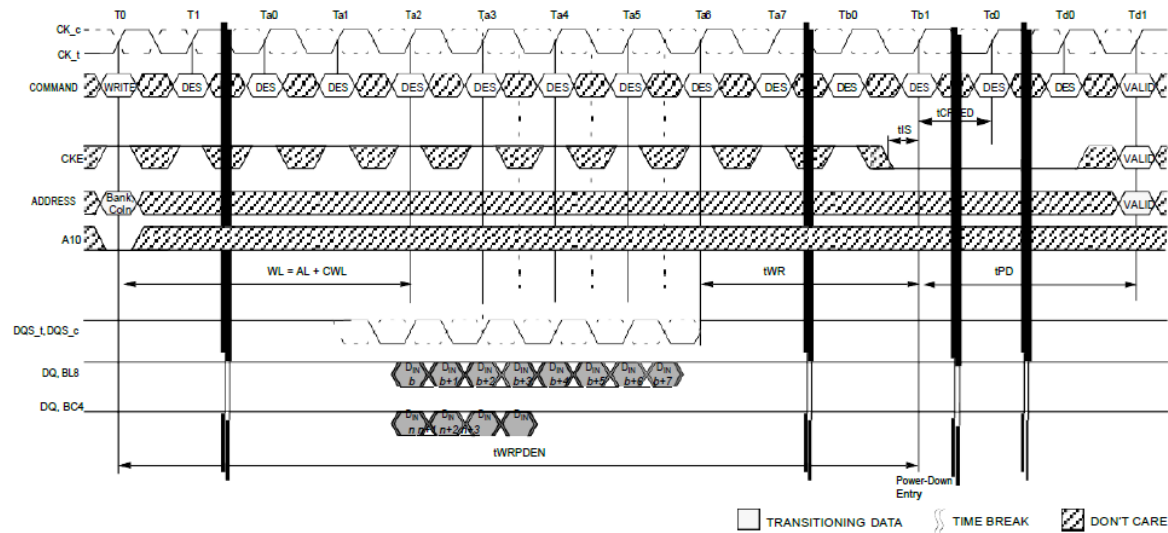
Power-Down Entry after Write
