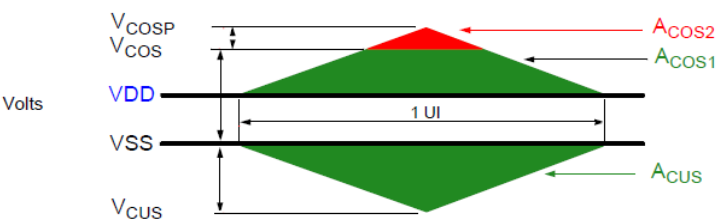
Clock Overshoot and Undershoot Definition
