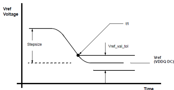
Vref step single stepsize decrement case
