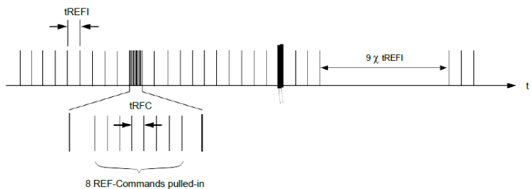
Pulling-in Refresh Commands (Example of 1X Refresh mode)
