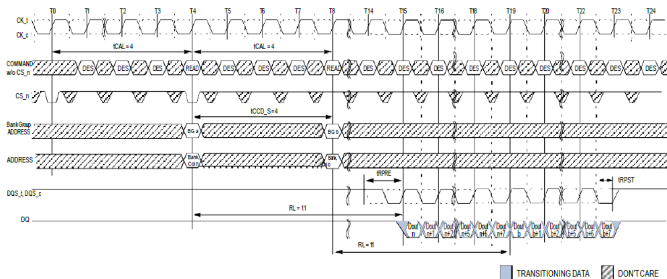
Consecutive READ (BL8) with CAL(4) and 1tCK Preamble in Different Bank Group
