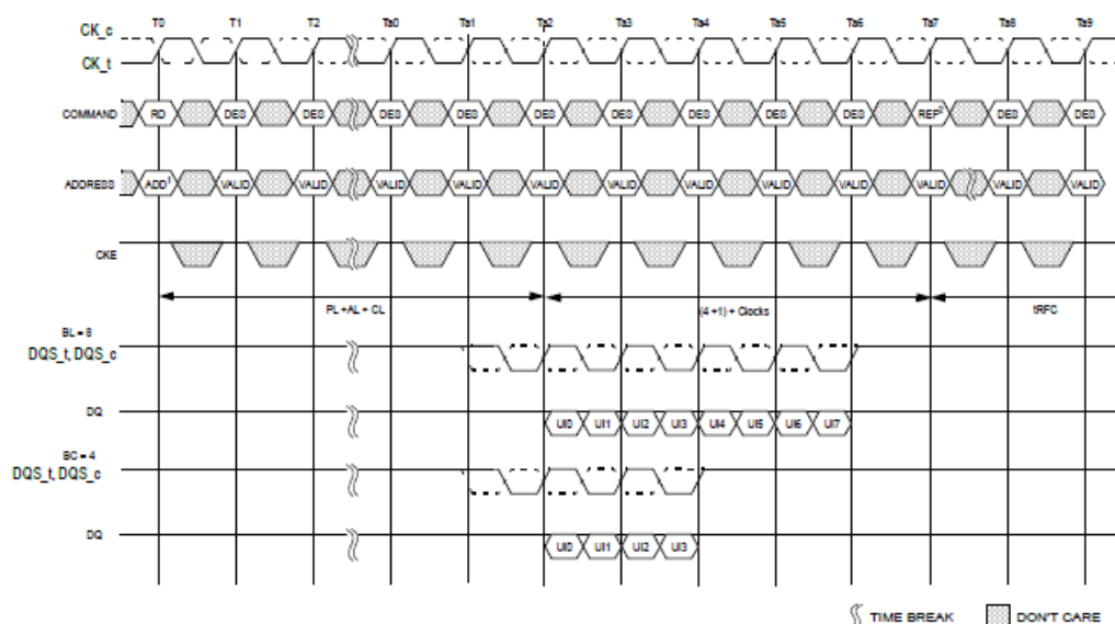
Read to Refresh Command Timing
