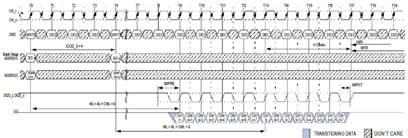
Consecutive WRITE (BL8) with 1tCK Preamble in Different Bank Group
