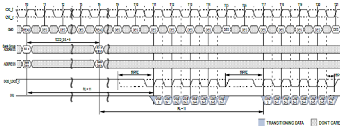
Nonconsecutive READ (BL8) with 2tCK Preamble in Same or Different Bank Group
