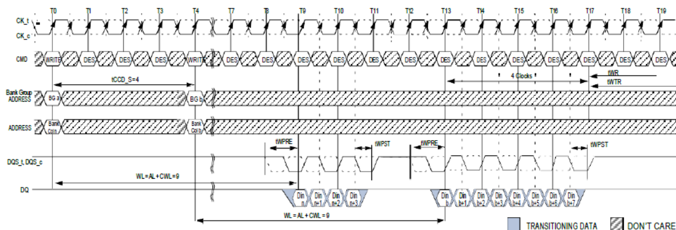
WRITE (BC4) OTF to WRITE (BL8) with 1tCK Preamble in Different Bank Group
