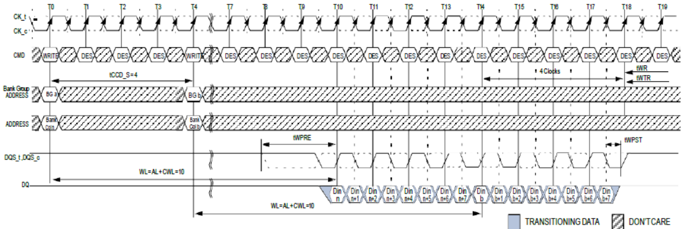
Consecutive WRITE (BL8) with 2tCK Preamble in Different Bank Group
