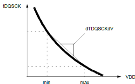
dTDQSCKdT Definition
