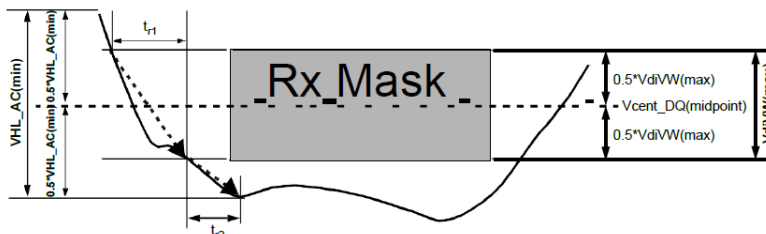
Slew Rate Conditions For Falling Transition
