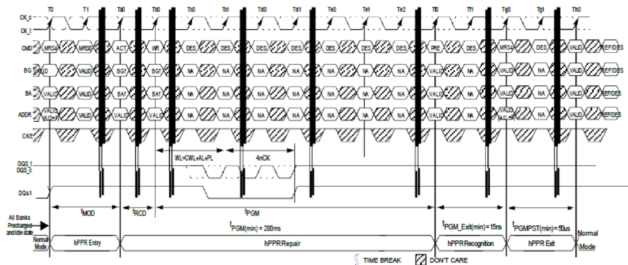
Hard Fail Row Repair (WR Case)
