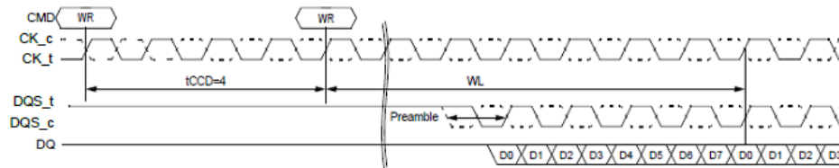
2tCK mode
