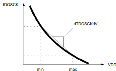
dTDQSCKdT Definition
