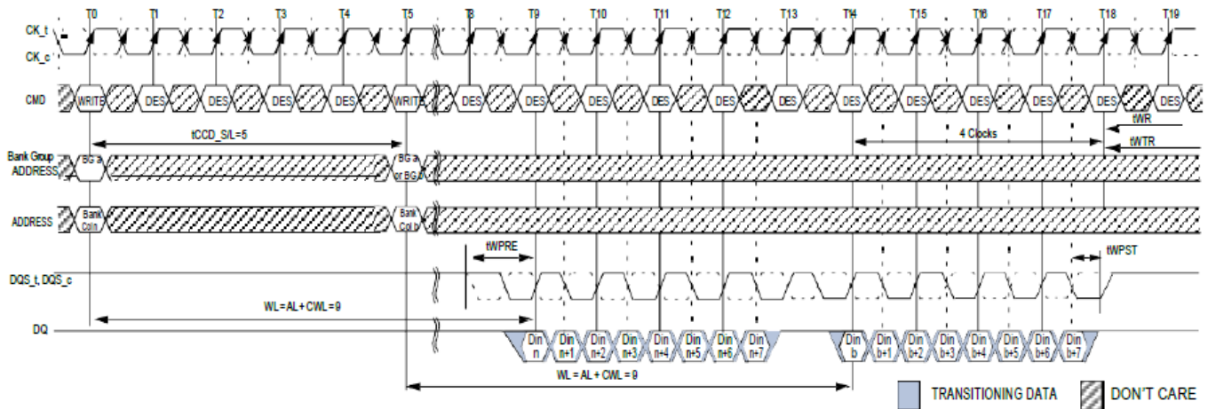
Nonconsecutive WRITE (BL8) with 1tCK Preamble in Same or Different Bank Group
