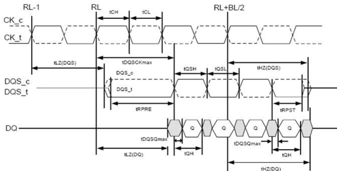
Figure of Data output (read) timing ( t_{DQSCK\ max} )
