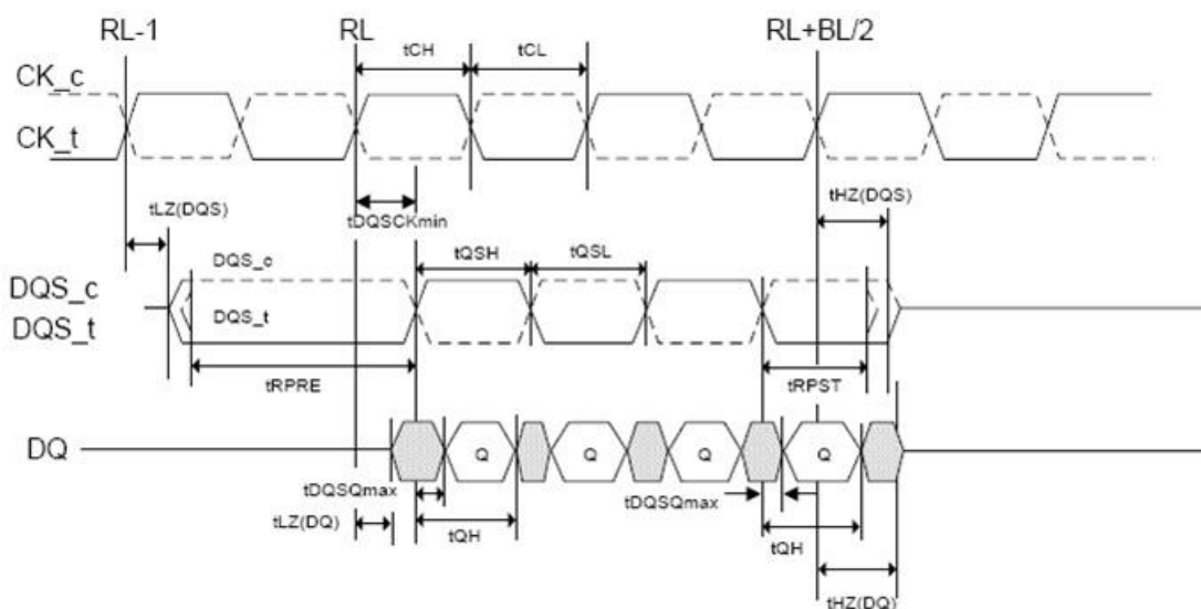
Figure of Data output (read) timing ( t_{DQSK\ min} )
