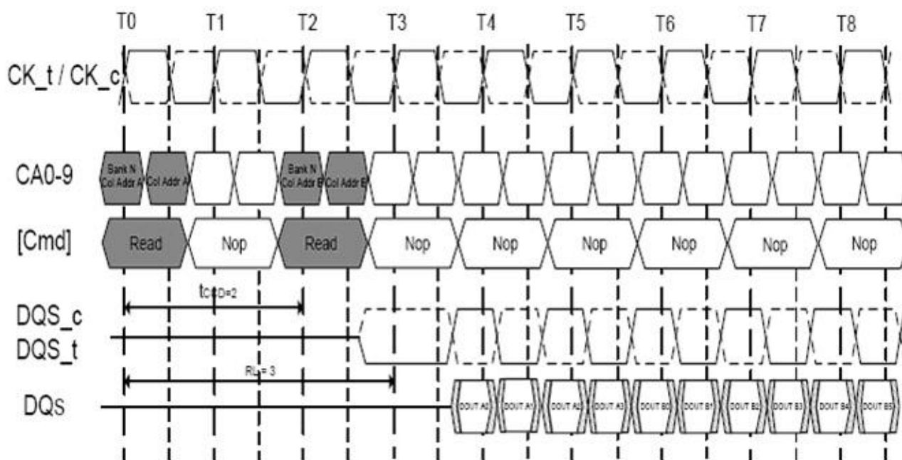
Figure of Read burst interrupt example: RL = 3 , BL = 8 , t_{CCD} = 2
