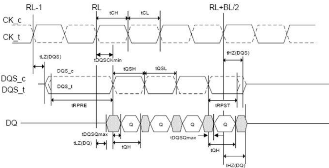
Figure of Data output (read) timing ( t_{DQCK\ min} )
