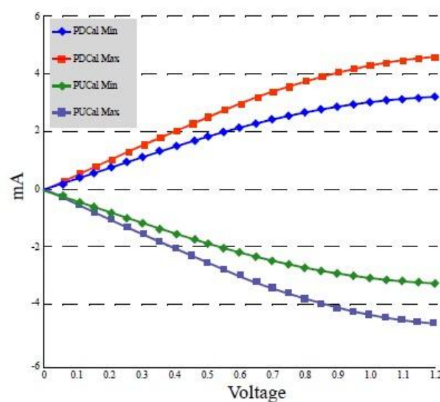
Figure of R_{ON} = 240\ \Omega IV Curve after calibration
