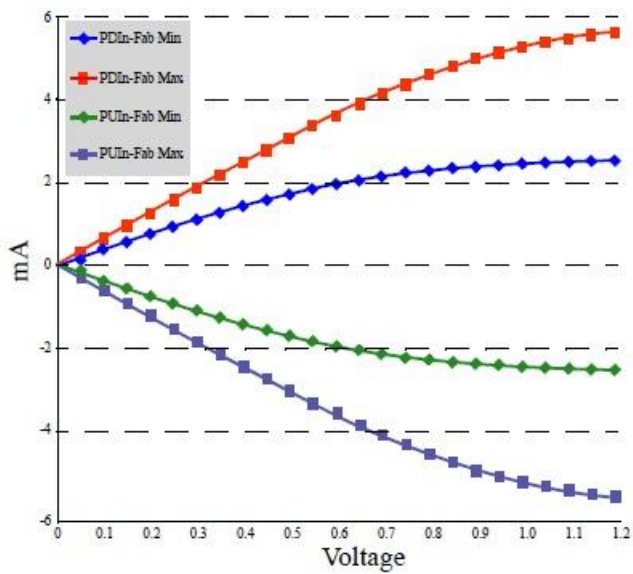
Figure of R_{ON} = 240\ \Omega IV Curve after ZQReset
