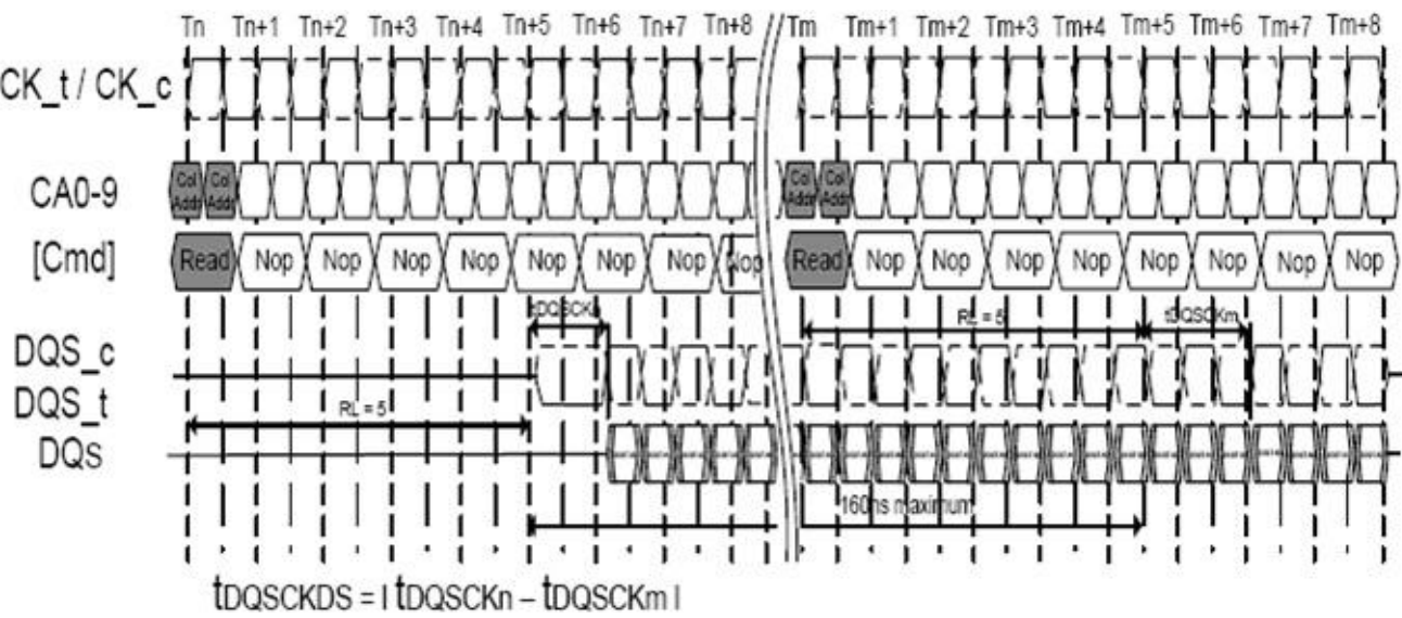
Figure of t_{DQCKDS} timing
