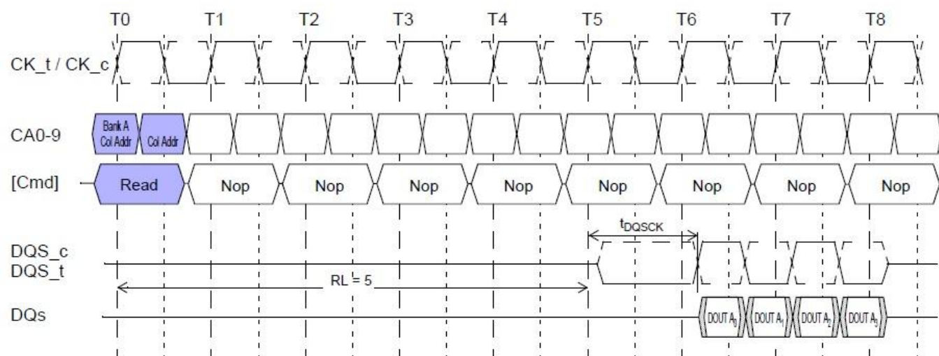
Figure of Burst read: RL = 5, BL = 4, t_{DQSCK} > t_{CK}
