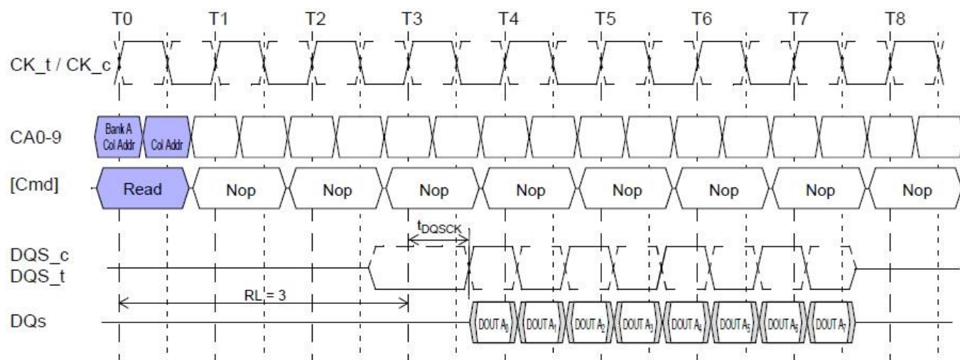
Figure of Burst read: RL = 3, BL = 8, t_{\text{BQSK}} < t_{\text{CK}}
