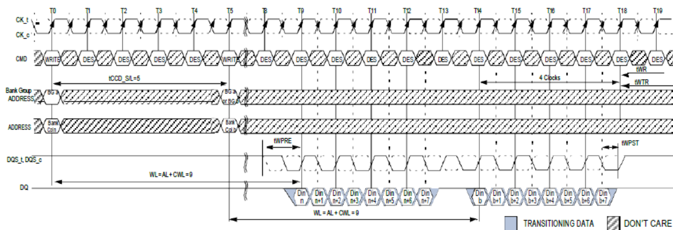
Nonconsecutive WRITE (BL8) with 1tCK Preamble in Same or Different Bank Group
