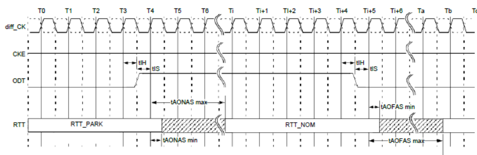
Asynchronous ODT Timing on DDR4 SDRAM with DLL-off
