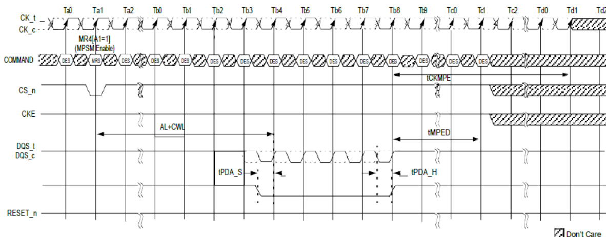
Maximum Power Saving mode Entry with PDA
