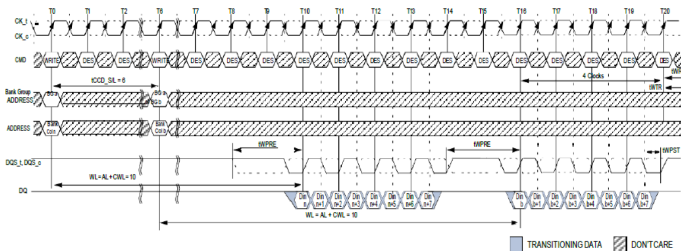
Nonconsecutive WRITE (BL8) with 2tCK Preamble in Same or Different Bank Group
