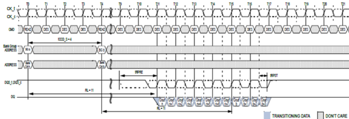
READ (BL8) to READ (BC4) OTF with 2tCK Preamble in Different Bank Group
