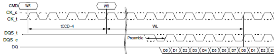
2tCK mode
