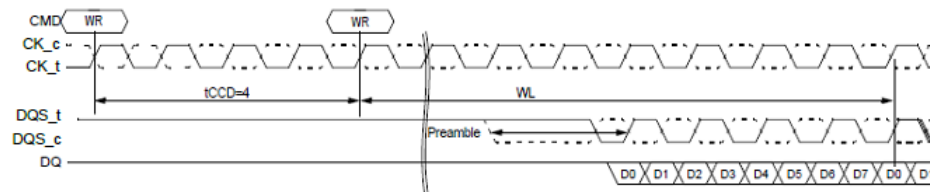
2tCK mode
