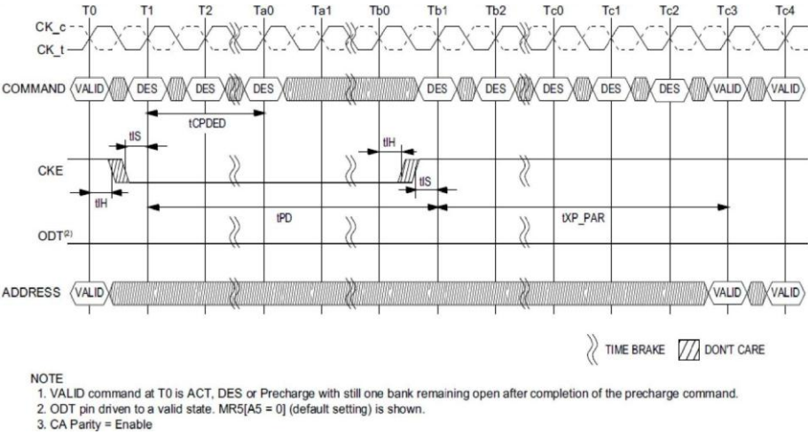
Power Down Entry and Exit Timing with C/A Parity
