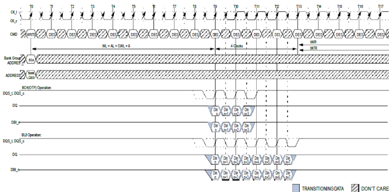
WRITE (BL8/BC4) OTF with 1tCK Preamble and DBI
