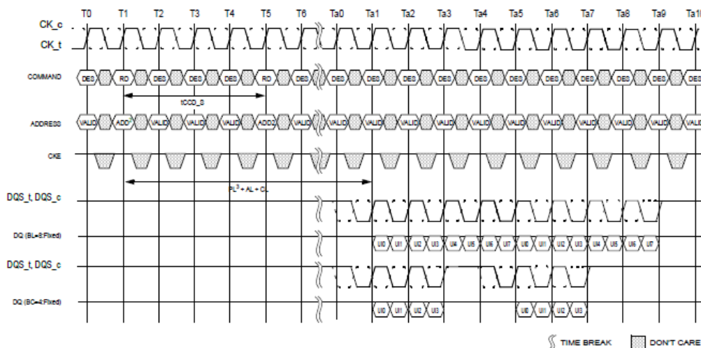
MPR Back to Back Read Timing
