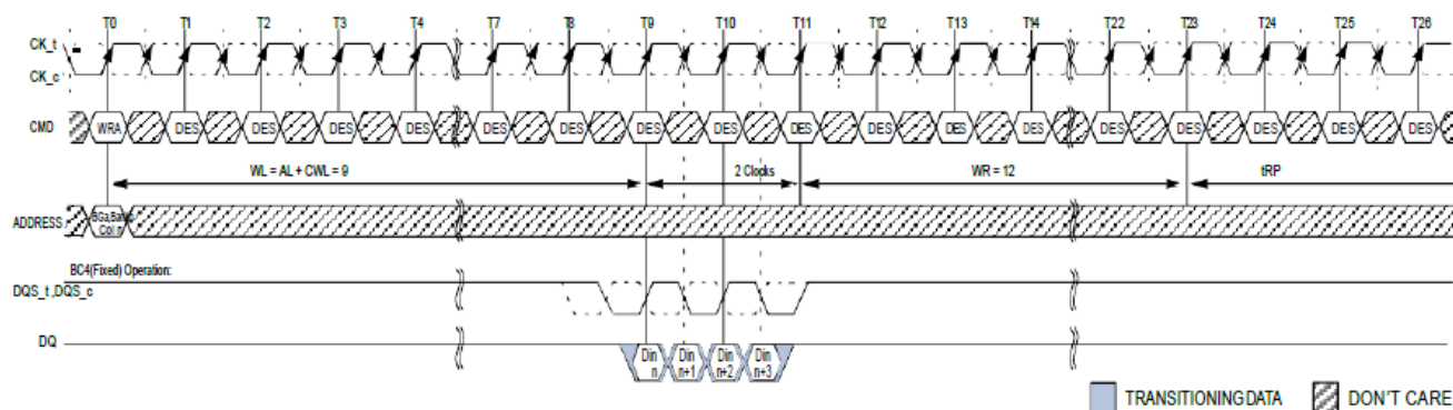
WRITE (BC4) Fixed with Auto PRECHARGE Operation and 1tCK Preamble
