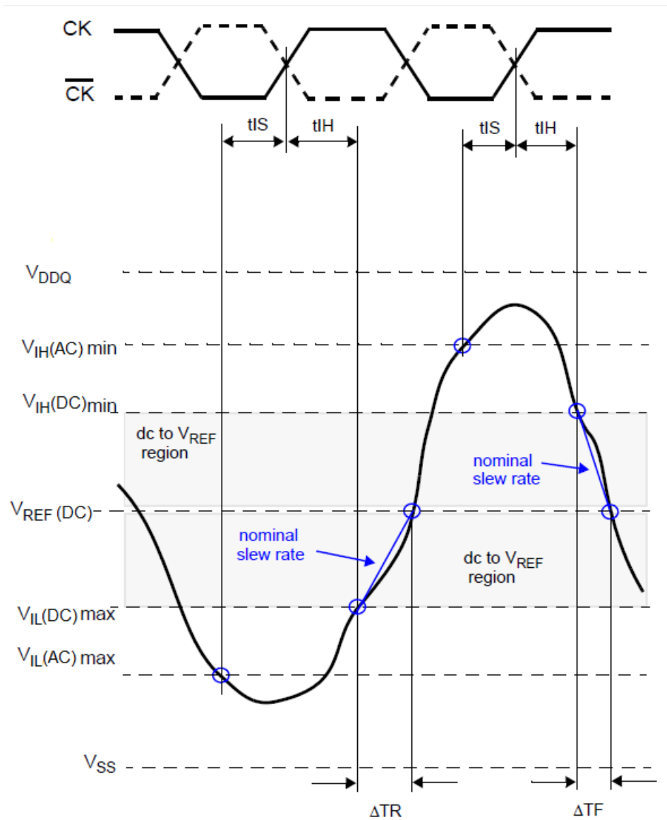
Illustration of nominal slew rate for hold time tIH (for ADD/CMD with respect to clock)
