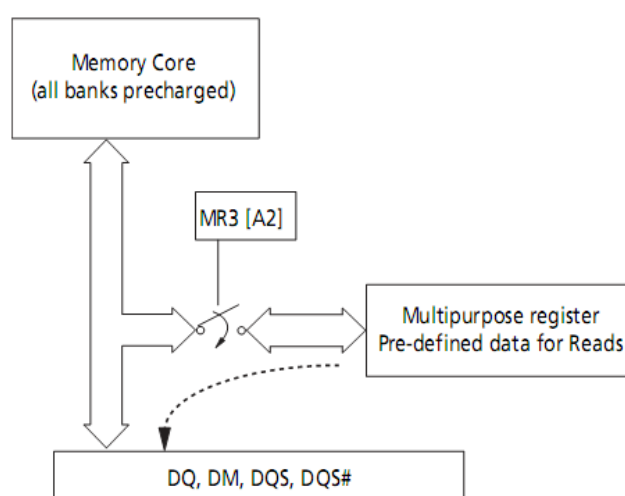
MPR Block Diagram
