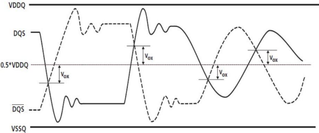
Definition of Output cross point voltage for DQS and \overline{\text{DQS}}
