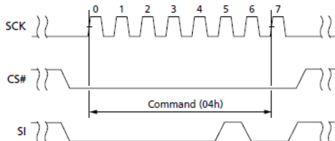
WRITE DISABLE (04h) Timing
