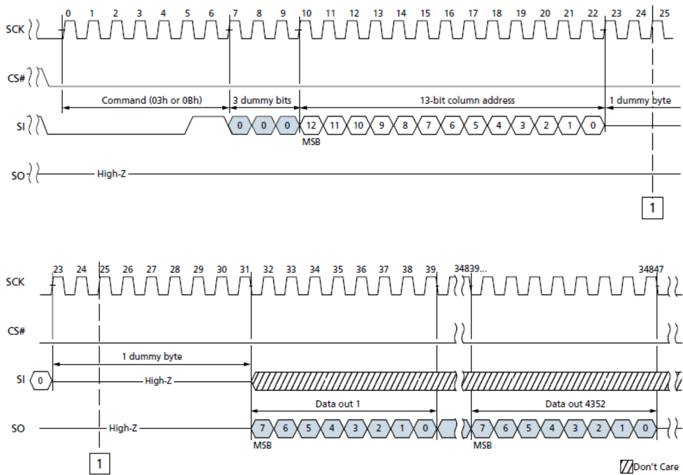
READ FROM CACHE (03h or 0Bh) Timing
