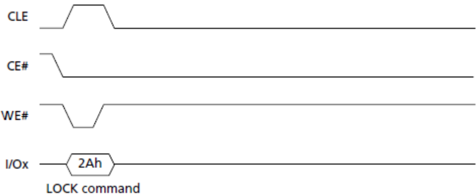
LOCK Operation
