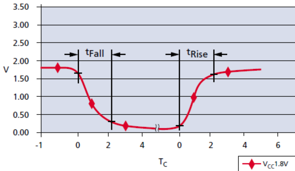
t Fall and t Rise
