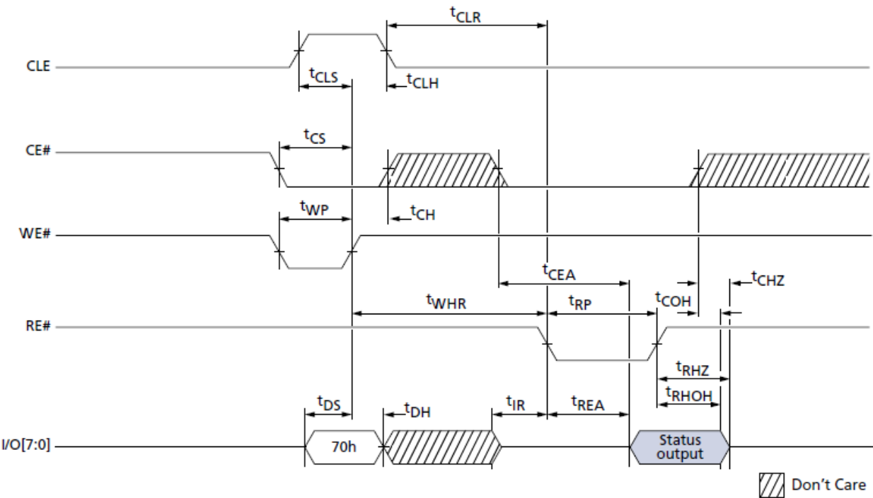
READ STATUS Cycle
