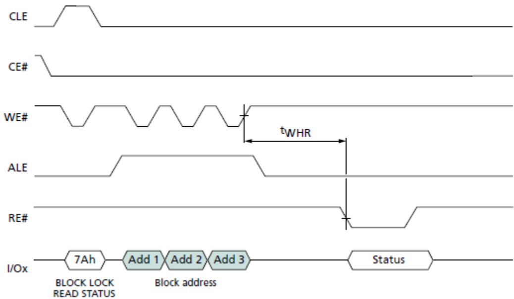
BLOCK LOCK READ STATUS
