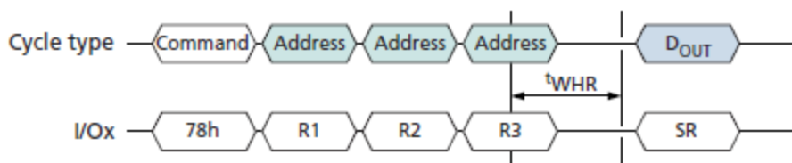
READ STATUS ENHANCED (78h) Operation
