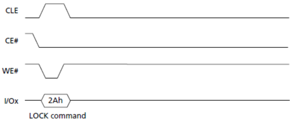
LOCK Operation
