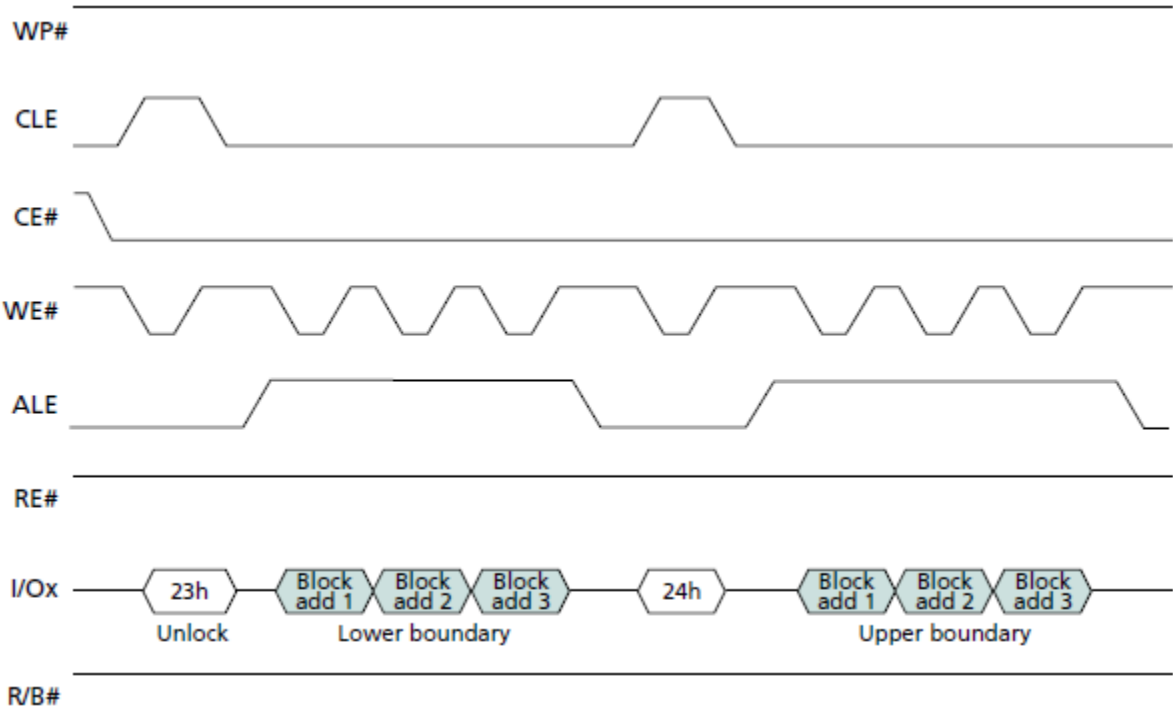
UNLOCK Operation
