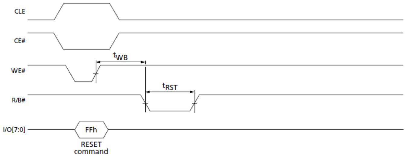
RESET Operation
