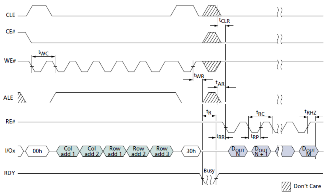
READ PAGE
