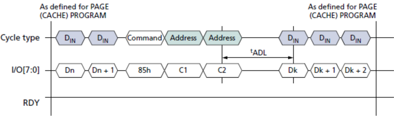
RANDOM DATA INPUT (85h) Operation
