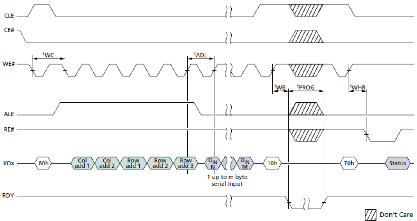
PROGRAM PAGE Operation
