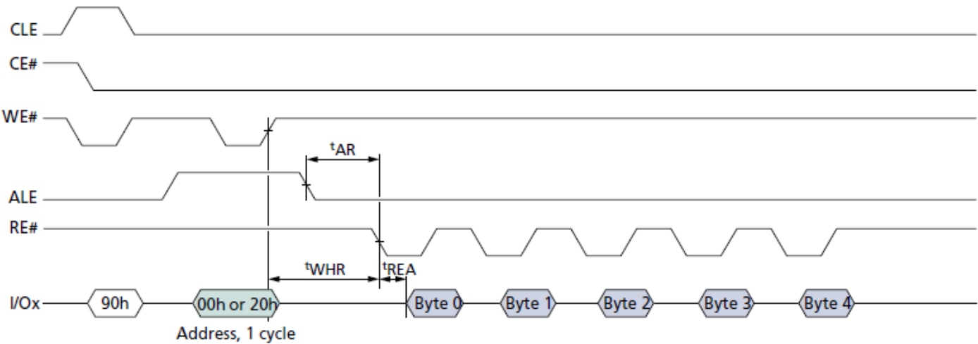
READ ID Operation
