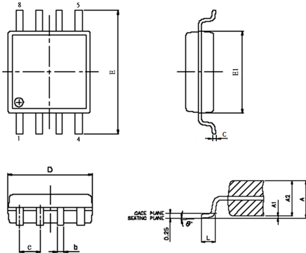
Figure 107. 8-pin SOP 200 mil (official name = 208 mil)
