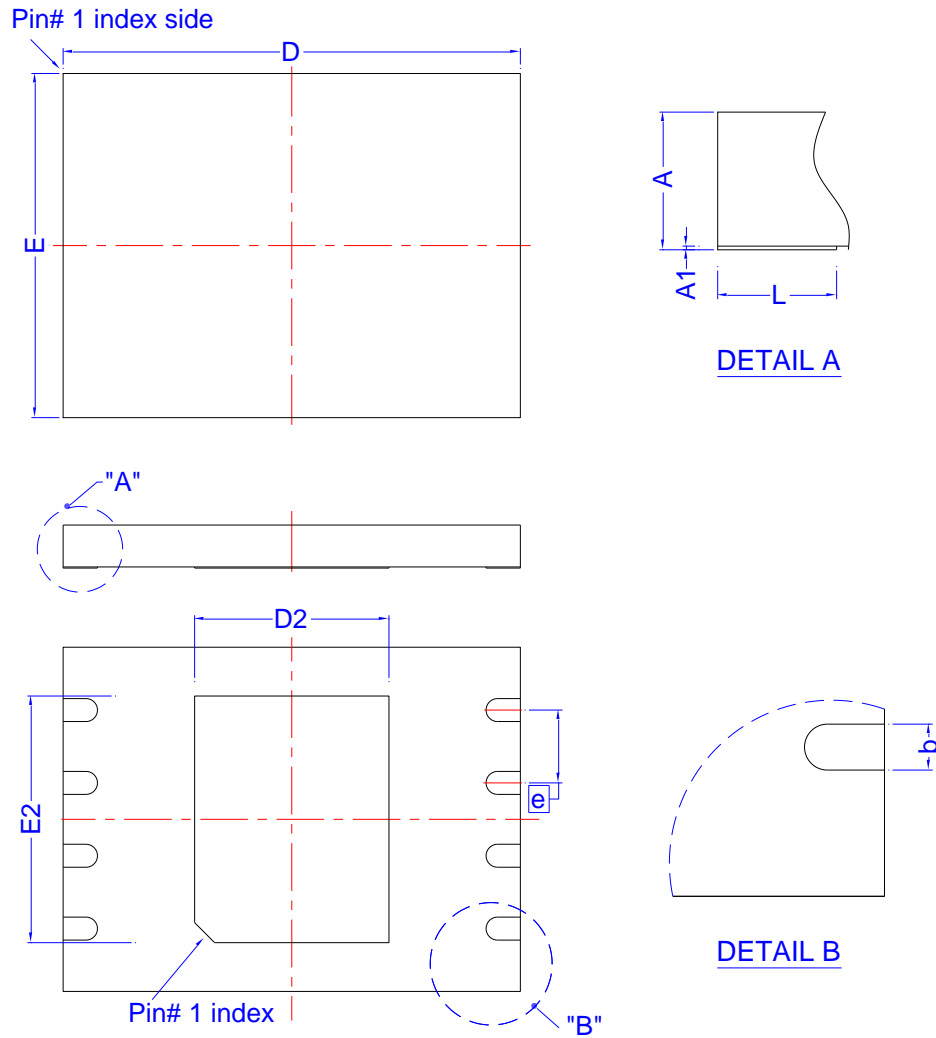
Figure 110. 8-contact VDFN / WSON (8x6 mm)
