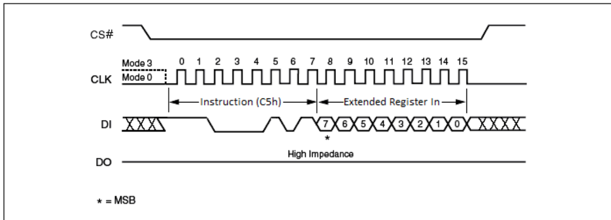
Figure 82. Write Extended Register Instruction Sequence Diagram
