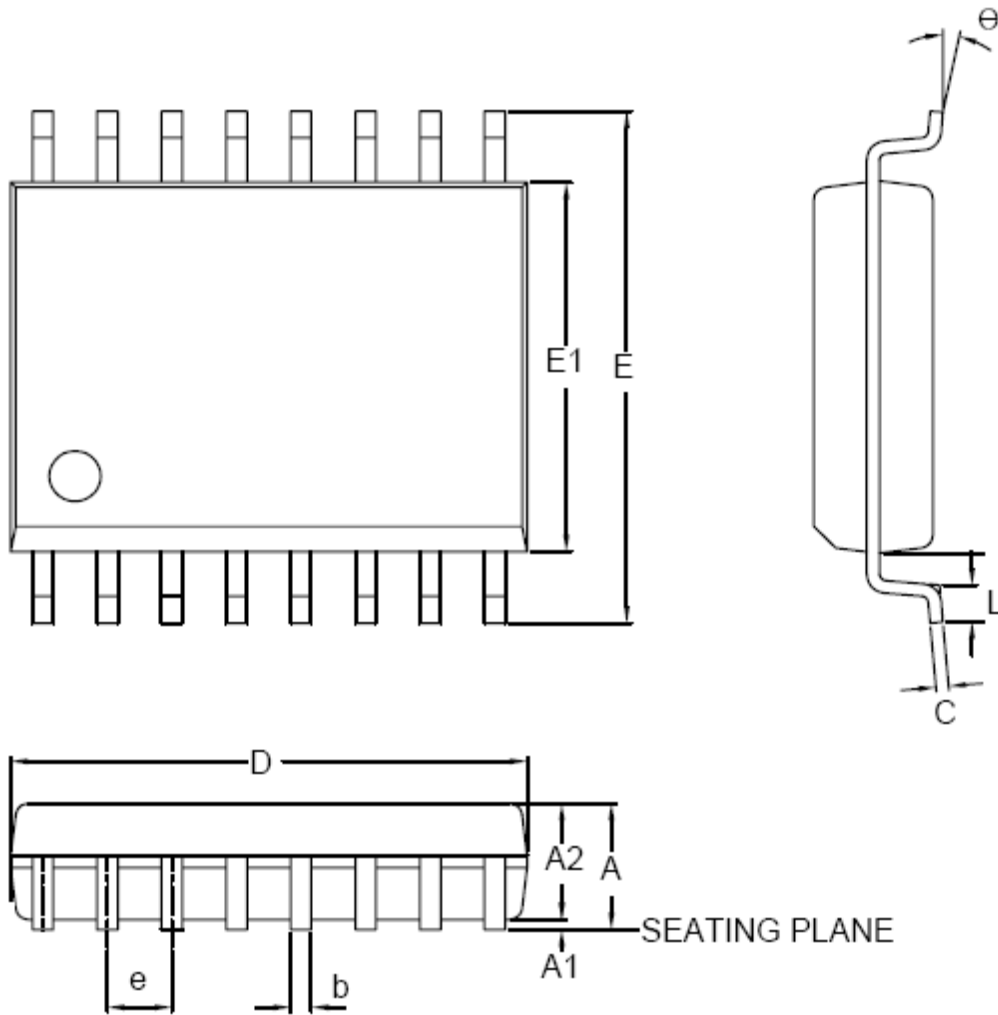
Figure 108. 16-pin SOP 300 mil
