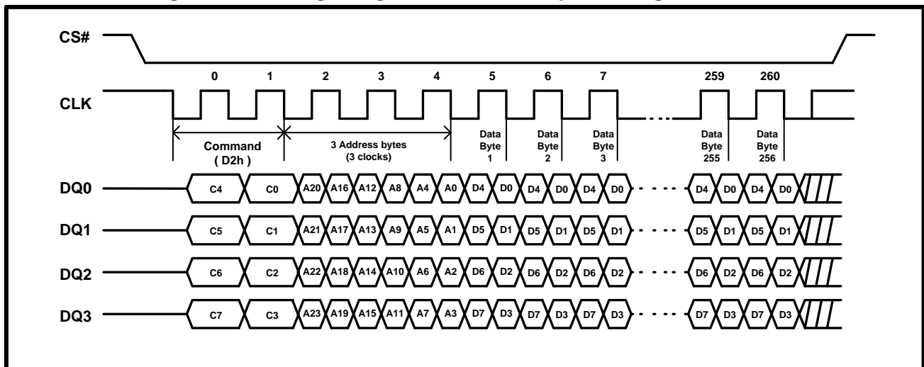
Figure 65. DDR Page Program Instruction Sequence Diagram in QPI Mode
