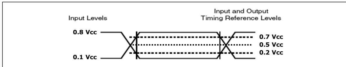
Figure 101. AC Measurement I/O Waveform
