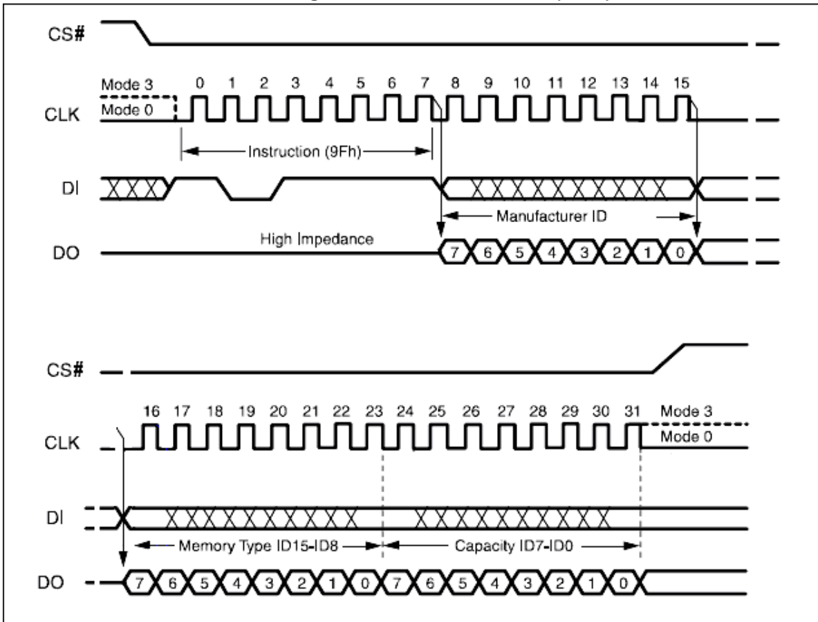
Figure 91. Read Identification (RDID)
