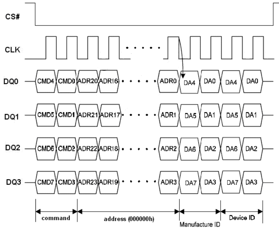
Figure 88. Read Manufacturer / Device ID Diagram in QPI Mode
