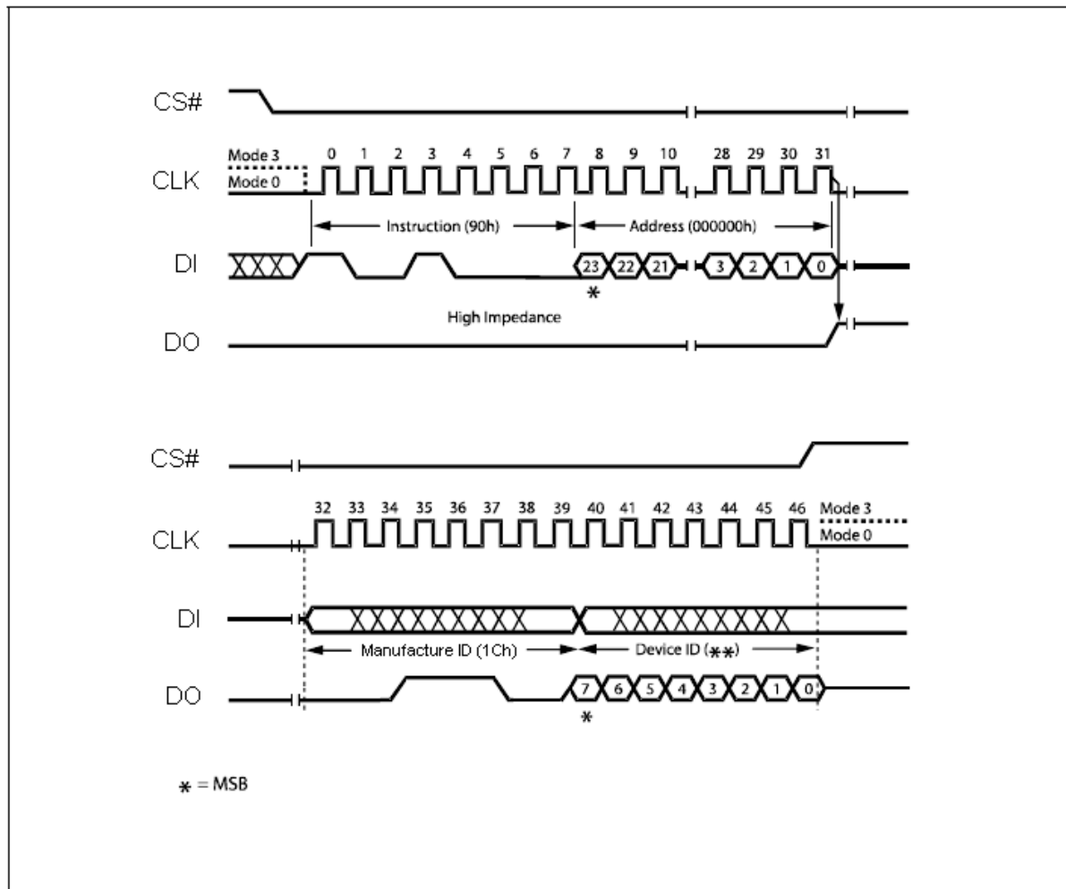
Figure 87. Read Manufacturer / Device ID Diagram
