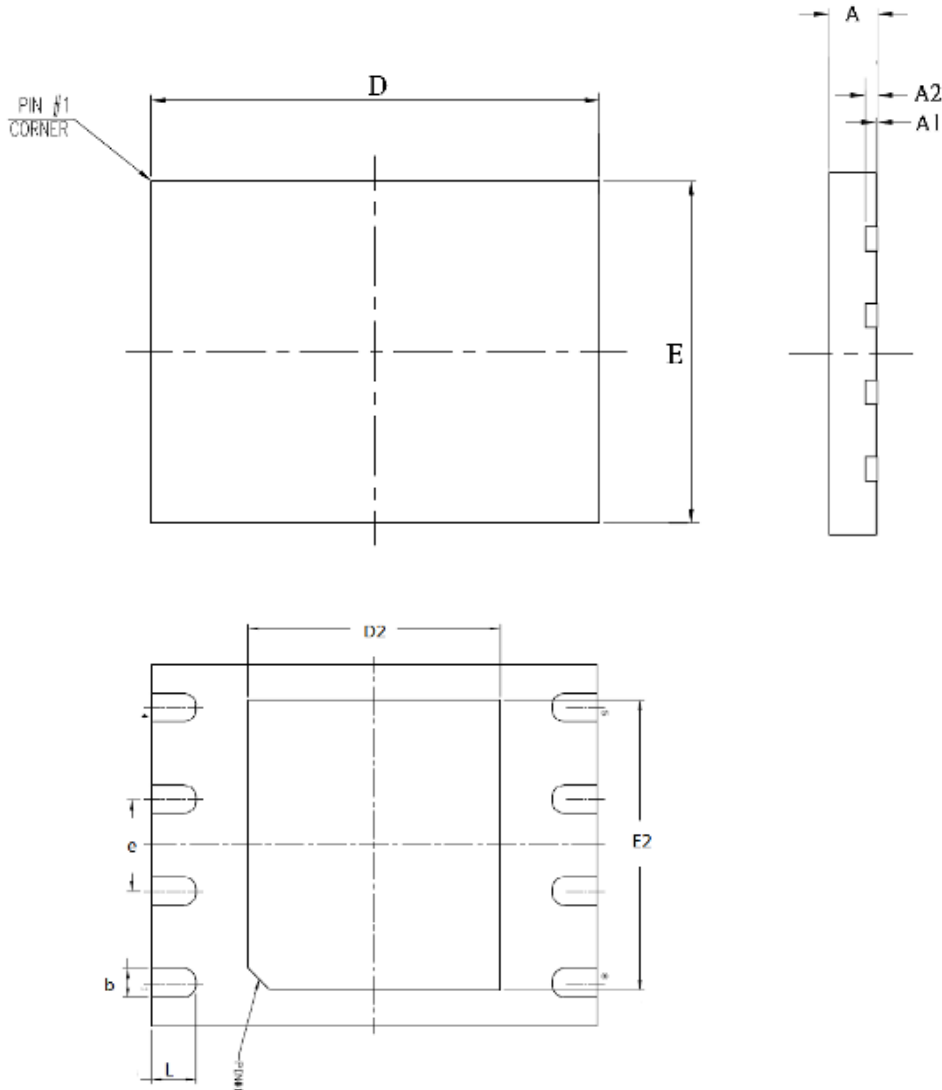
Figure 110. 8-contact VDFN / WSON (6x5 mm)
