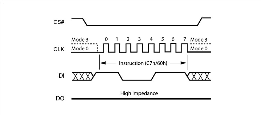
Figure 74. Chip Erase Instruction Sequence Diagram
