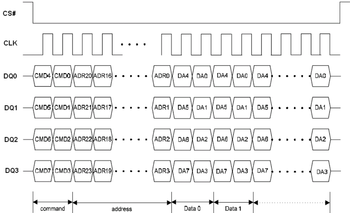
Figure 94. Program OTP array (QPI mode)
