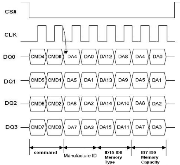
Figure 92. Read Identification (RDID) in QPI Mode
