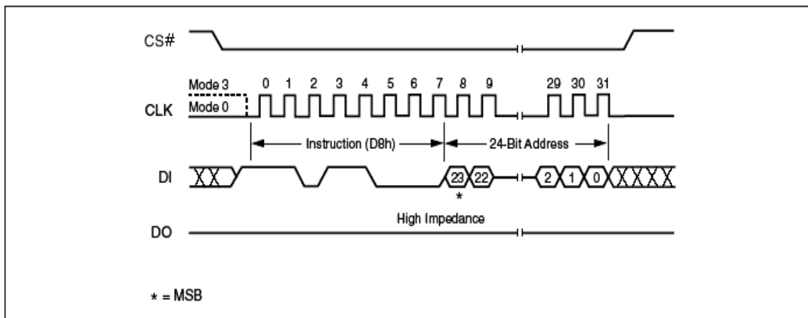
Figure 68. 64KB Block Erase Instruction Sequence Diagram
