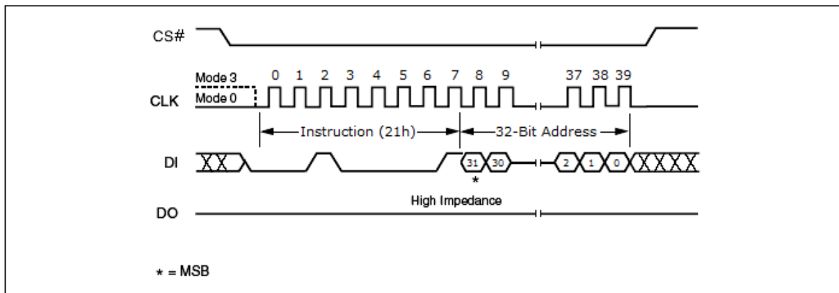
Figure 70. Sector Erase with 4byte address Instruction Sequence Diagram
