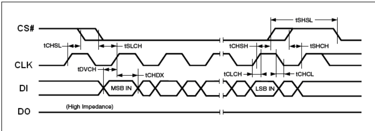
Figure 103. Input Timing
