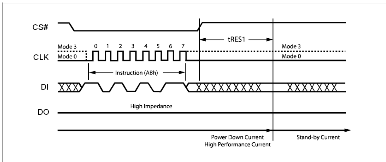
Figure 85. Release Power-down Instruction Sequence Diagram
