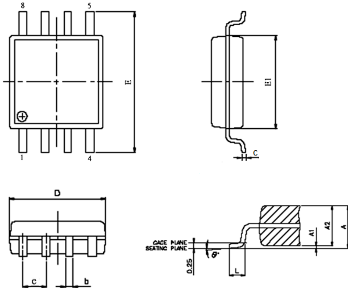
Figure 108. 8-pin SOP 200 mil (official name = 208 mil)
