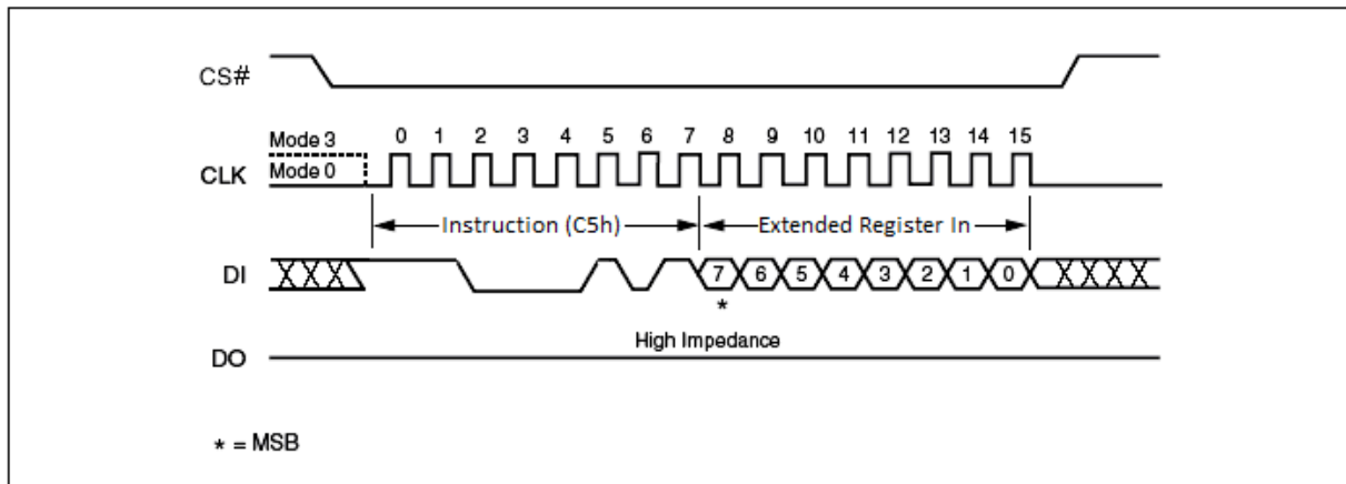
Figure 82. Write Extended Register Instruction Sequence Diagram
