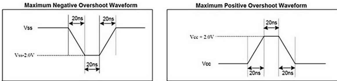
Figure 107. Overshoot Waveform
