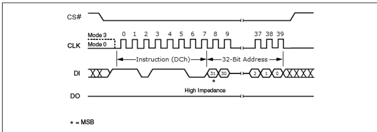
Figure 72. 64KB Block Erase with 4byte address Instruction Sequence Diagram
