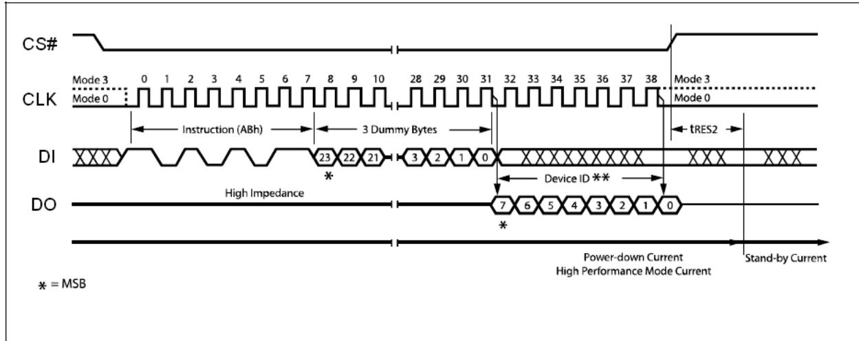
Figure 86. Release Power-down / Device ID Instruction Sequence Diagram
