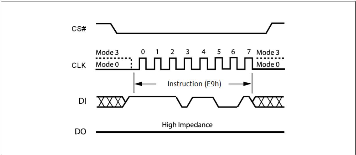
Figure 78. Exit 4byte address mode Instruction Sequence Diagram
