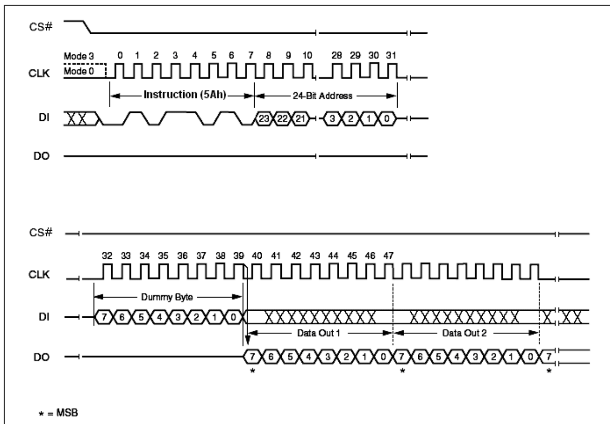
Figure 99. Read SFDP Mode and Unique ID Number Instruction Sequence Diagram
