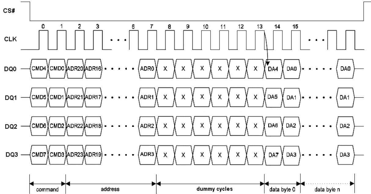
Figure 96. Read OTP array (QPI mode)
