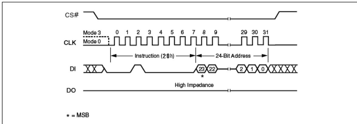
Figure 66. Sector Erase Instruction Sequence Diagram
