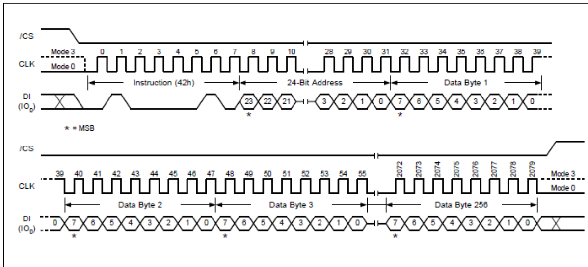
Figure 93. Program OTP array
