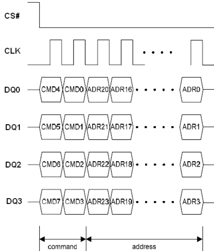
Figure 69. Block/Sector Erase Instruction Sequence in QPI Mode
