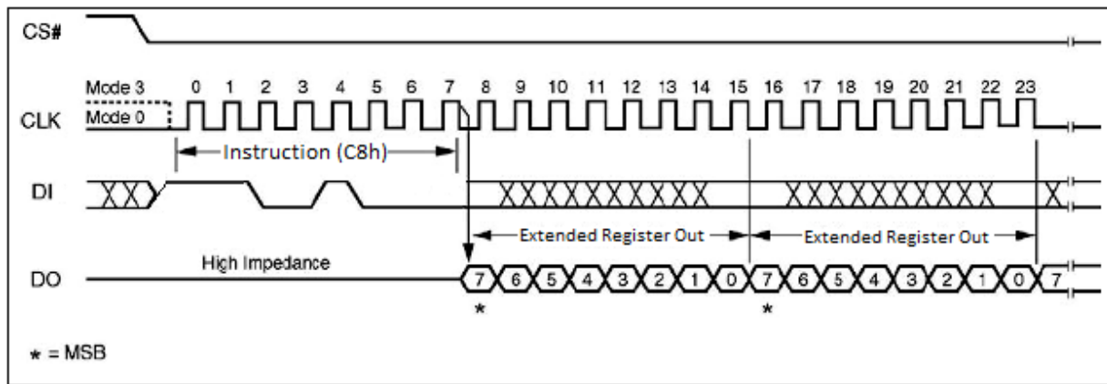
Figure 80. Read Extended Address Register Instruction Sequence Diagram
