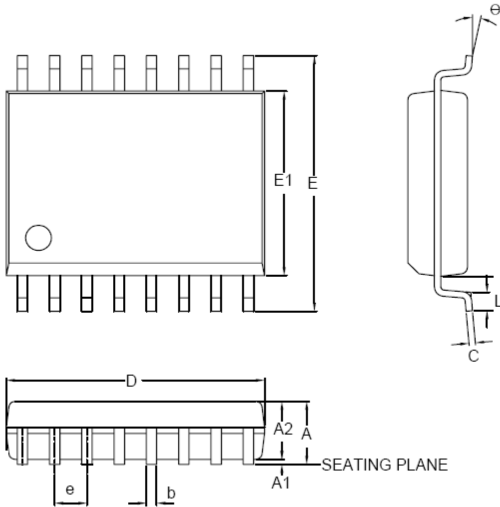
Figure 109. 16-pin SOP 300 mil
