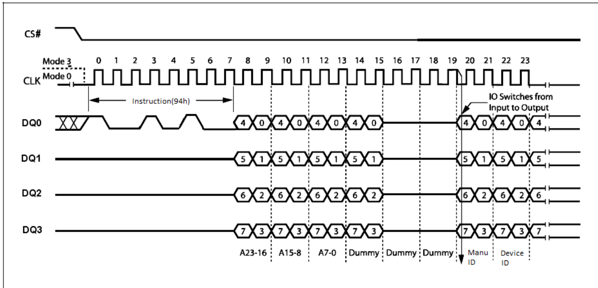
Figure 90. Read Manufacturer / Device ID by Quad I/O Diagram
