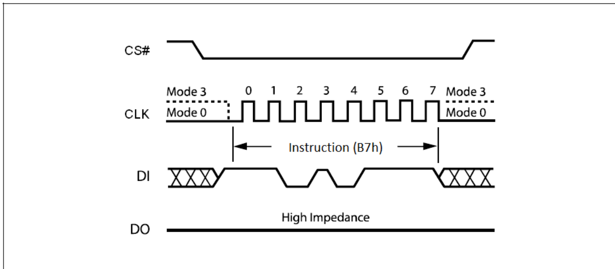
Figure 76. Enter 4byte address mode Instruction Sequence Diagram
