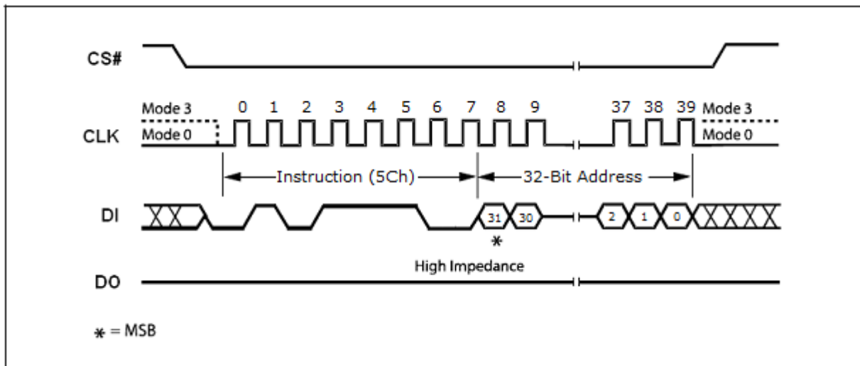
Figure 71. 32KB Half Block Erase with 4byte address Instruction Sequence Diagram
