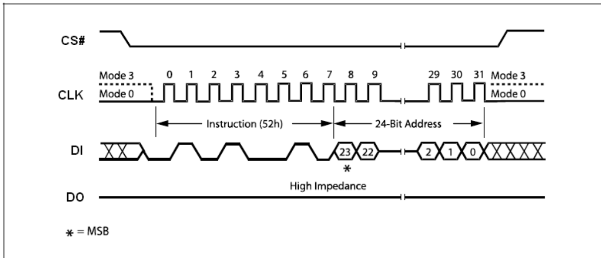
Figure 67. 32KB Half Block Erase Instruction Sequence Diagram
