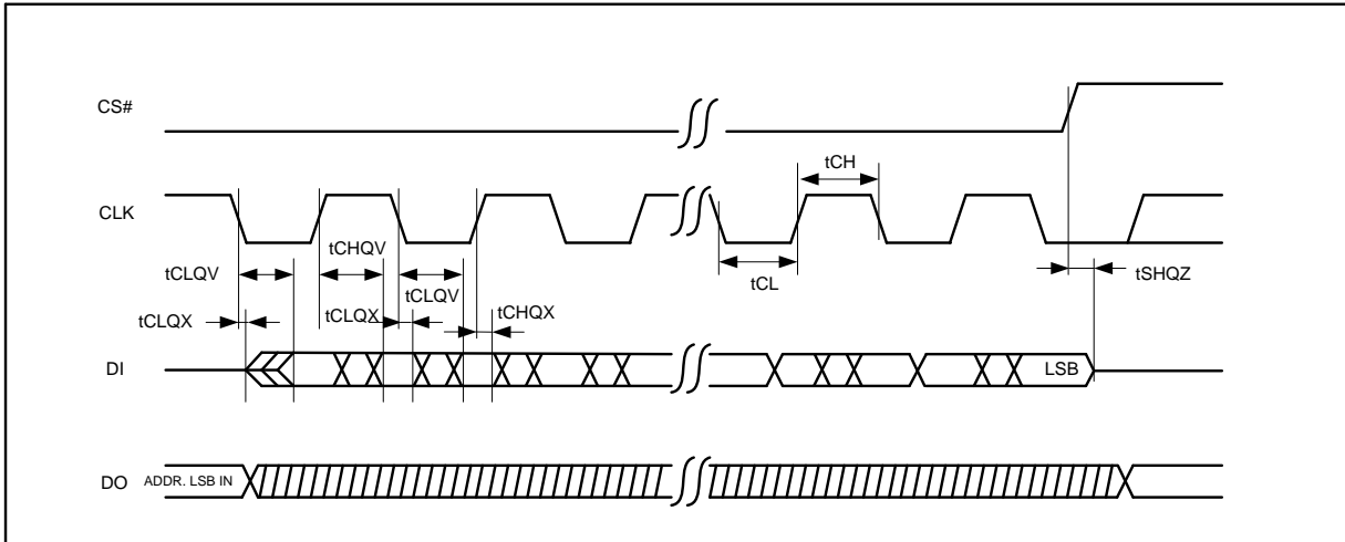
Figure 105. Serial Output Timing for Double Data Rate Mode
