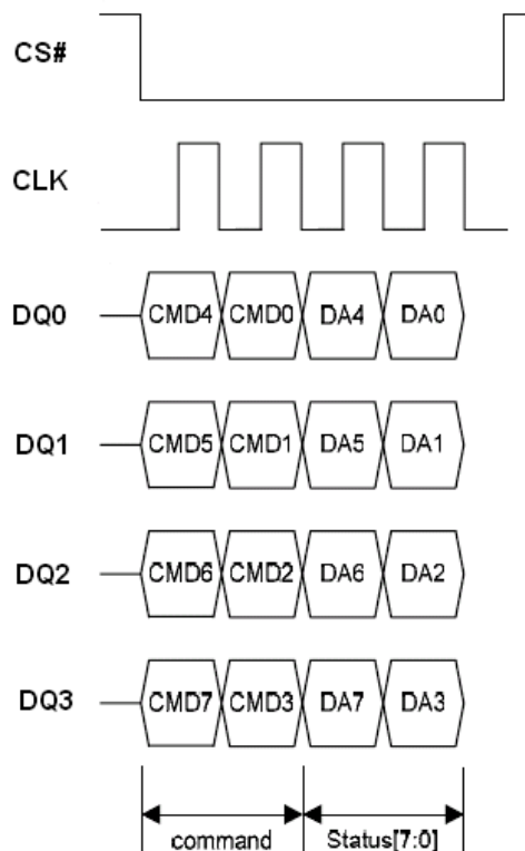
Figure 83. Write Extended Register Instruction Sequence in QPI Mode
