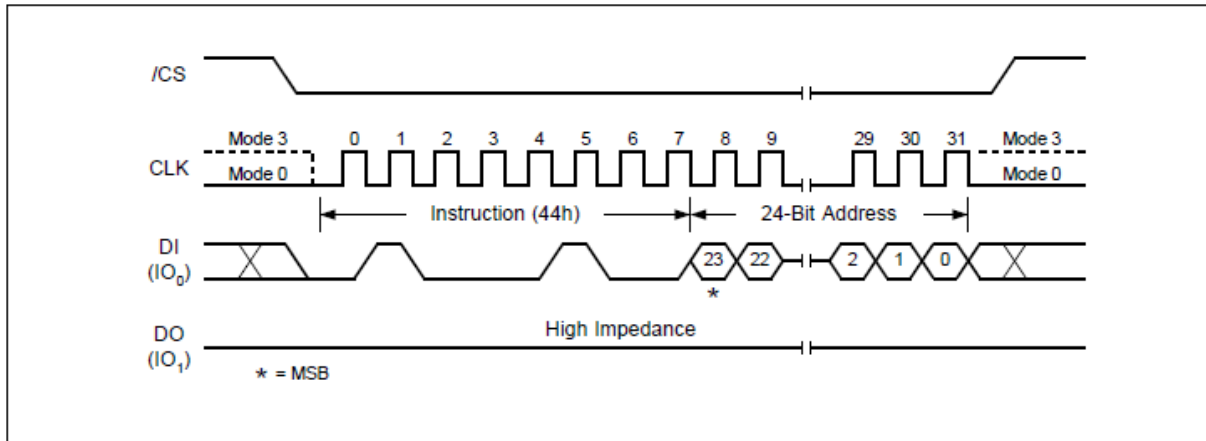
Figure 97. Erase OTP array
