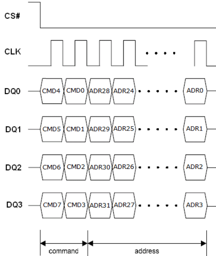
Figure 73. Block/Sector Erase with 4byte address Instruction Sequence in QPI Mode
