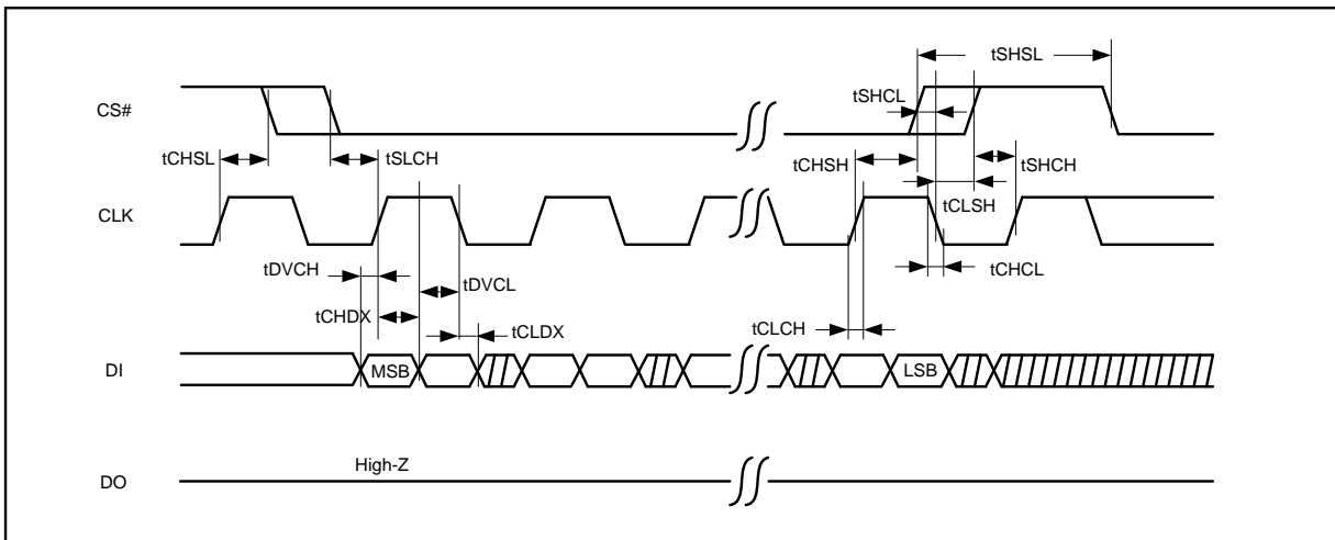
Figure 106. Serial Input Timing for Double Data Rate Mode
