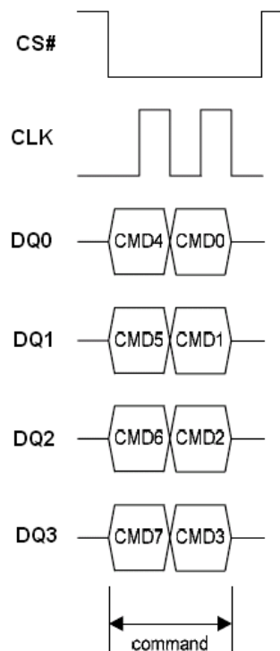
Figure 77. Enter 4byte address mode Sequence under EQPI Mode
