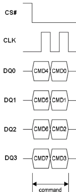
Figure 75. Chip Erase Sequence under EQPI Mode
