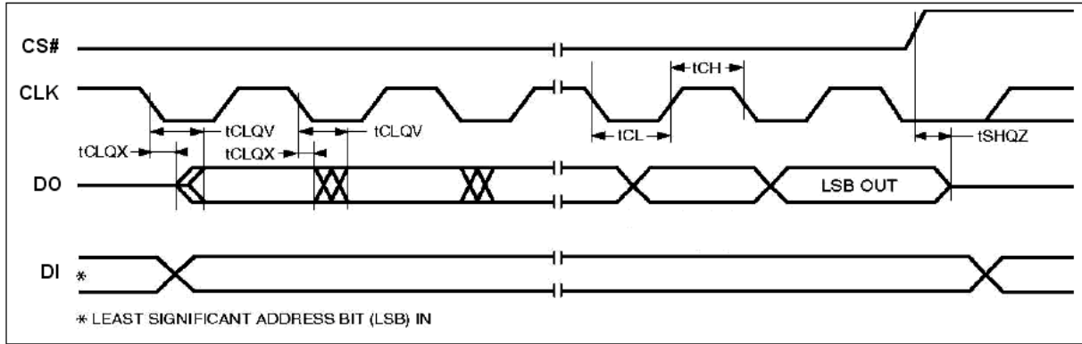
Figure 102. Serial Output Timing
