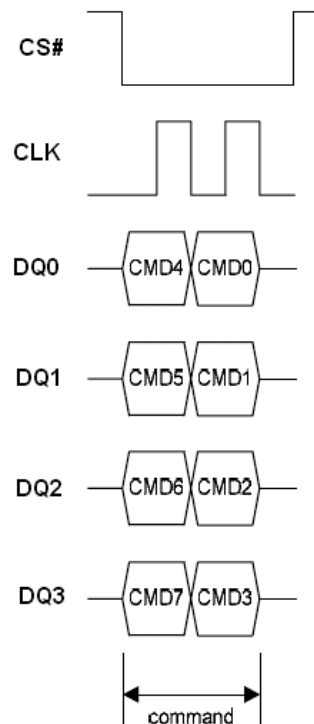
Figure 79. Exit 4byte address mode Sequence under EQPI Mode
