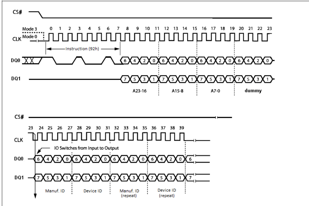
Figure 89. Read Manufacturer / Device ID by Dual I/O Diagram
