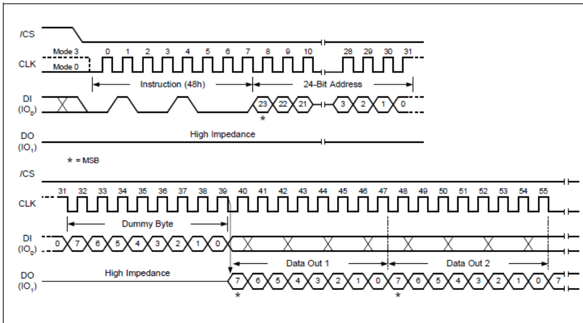
Figure 95. Read OTP array
