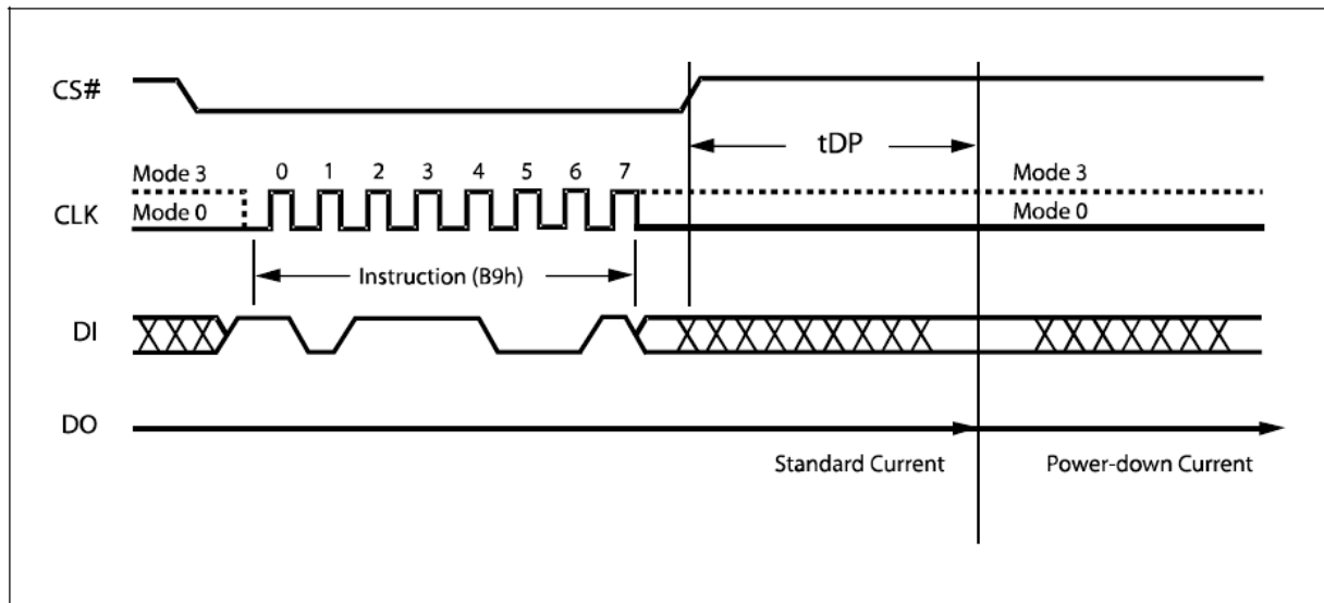
Figure 84. Deep Power-down Instruction Sequence Diagram
