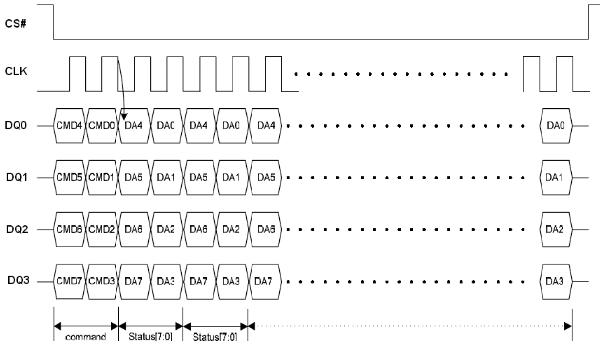
Figure 81. Read Extended Address Register Instruction Sequence under QPI Mode
