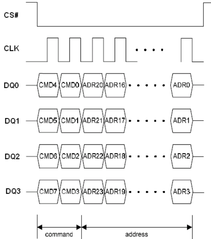
Figure 98. Erase OTP array (QPI mode)
