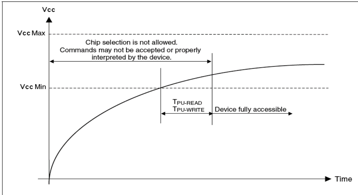
Figure 100. Power-up Timing
