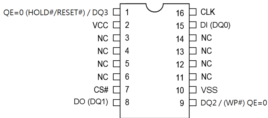
16 – LEAD SOP
