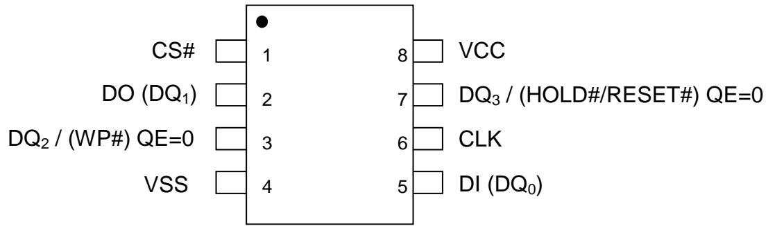
8 – LEAD SOP
