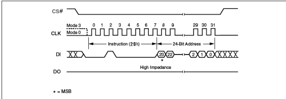
Sector Erase Instruction Sequence Diagram
