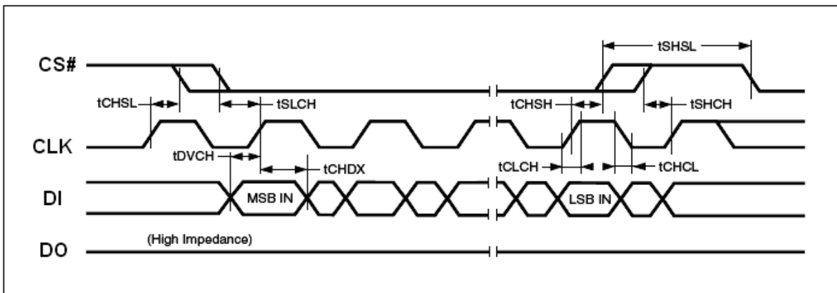
Input Timing
