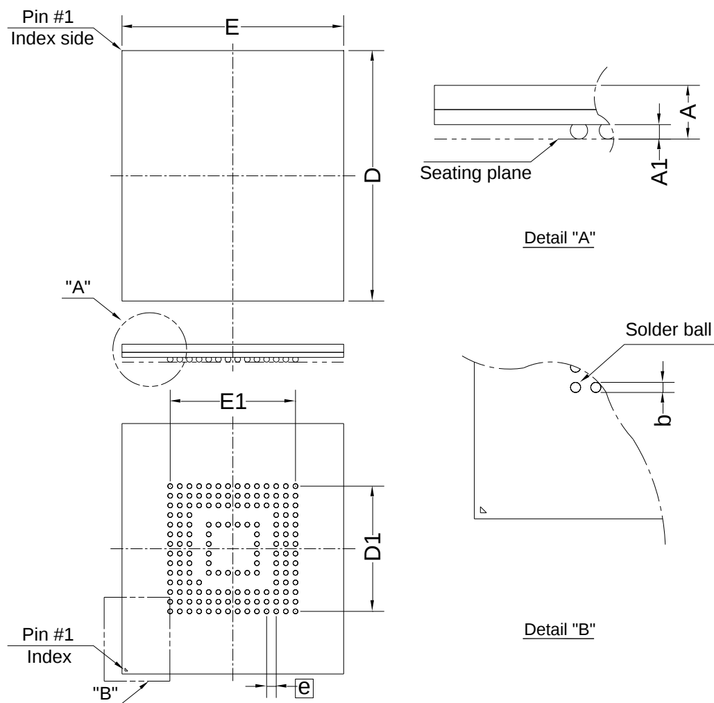
Figure 11. 153-BALL (11.5x13 mm)
